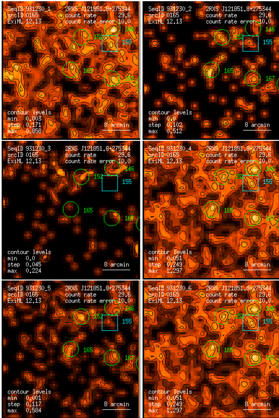
Figure 165: RASS 931230: detection 0165: band rate images, Gaussian filter: (1) PSPC channels 11 – 41, (2) 52 – 90, (3) 91 – 201, (4) 11 – 235, (5) 52 – 201, (6) 11 – 201. Broad band rates in counts/ks. Band rate contour levels in counts/ks/arcmin 2 .
