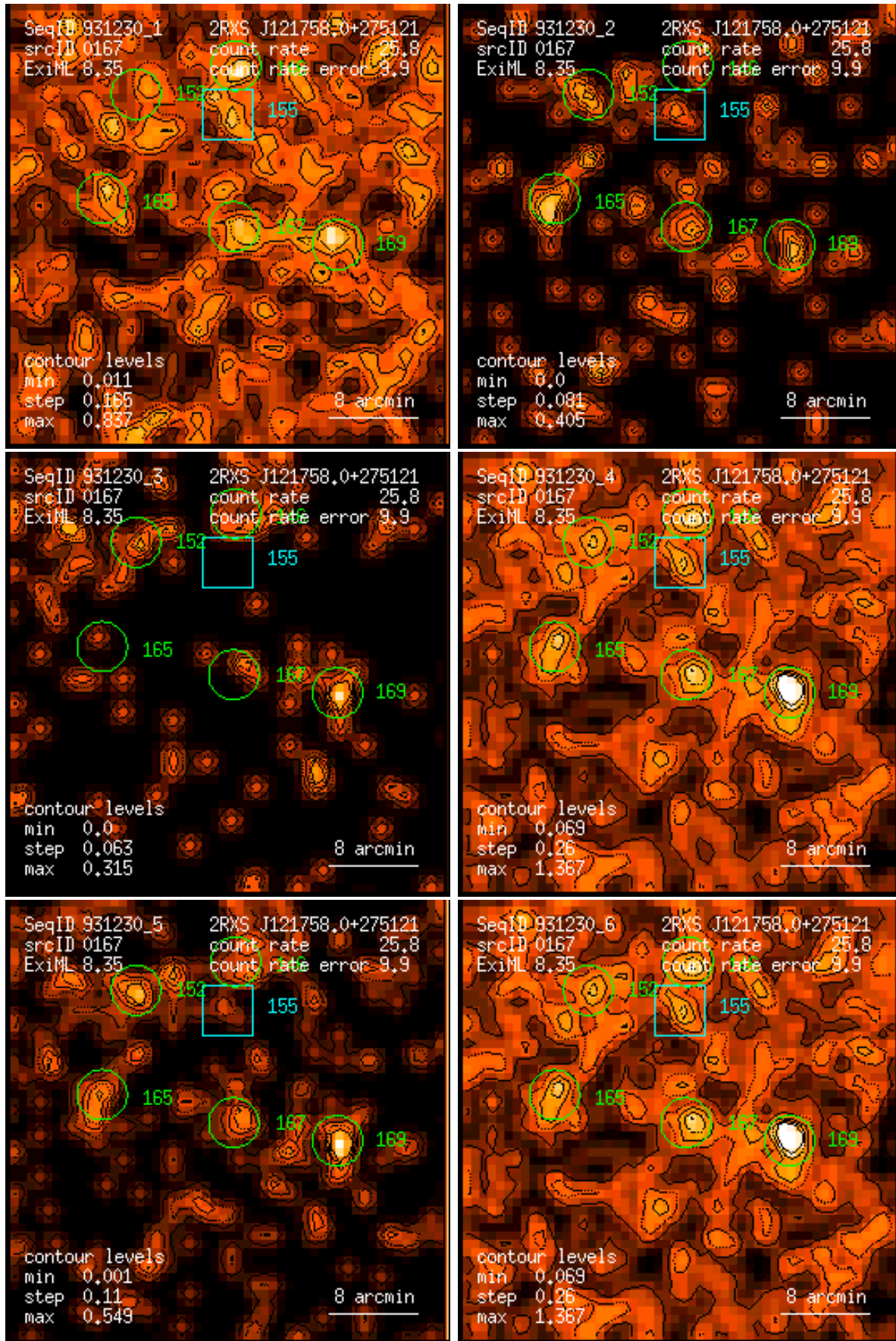
Figure 167: RASS 931230: detection 0167: band rate images, Gaussian filter: (1) PSPC channels 11 – 41, (2) 52 – 90, (3) 91 – 201, (4) 11 – 235, (5) 52 – 201, (6) 11 – 201. Broad band rates in counts/ks. Band rate contour levels in counts/ks/arcmin 2 .
