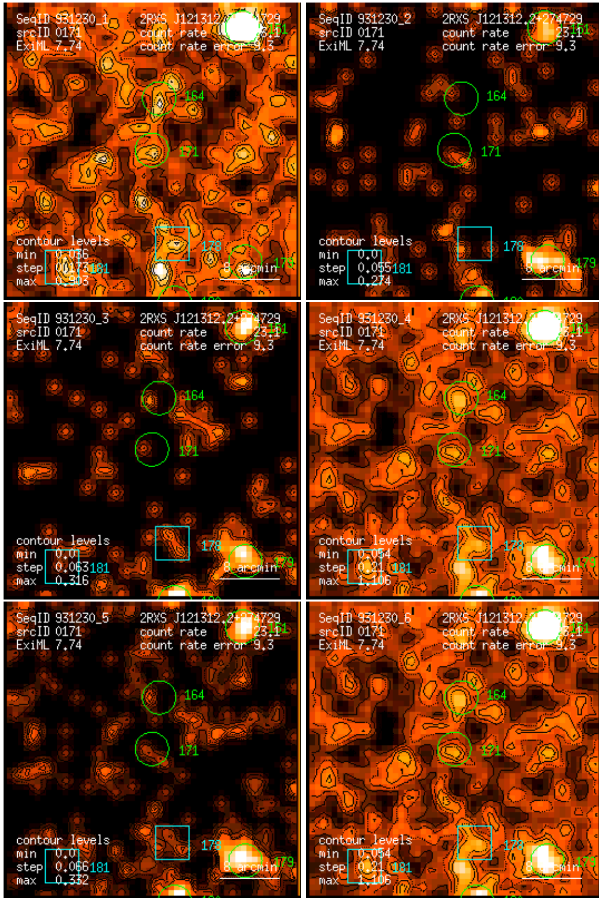
Figure 171: RASS 931230: detection 0171: band rate images, Gaussian filter: (1) PSPC channels 11 – 41, (2) 52 – 90, (3) 91 – 201, (4) 11 – 235, (5) 52 – 201, (6) 11 – 201. Broad band rates in counts/ks. Band rate contour levels in counts/ks/arcmin 2 .
