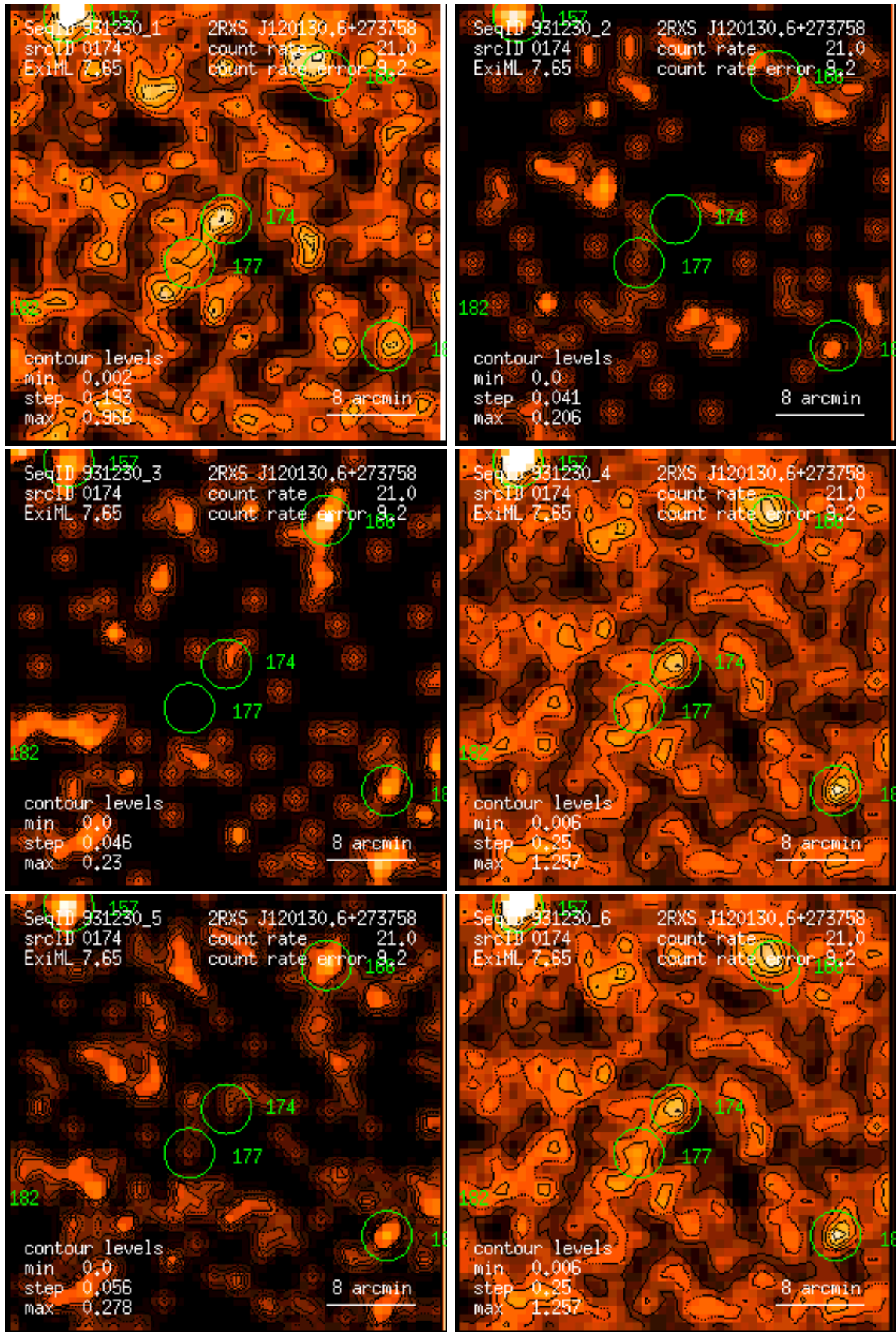
Figure 174: RASS 931230: detection 0174: band rate images, Gaussian filter: (1) PSPC channels 11 – 41, (2) 52 – 90, (3) 91 – 201, (4) 11 – 235, (5) 52 – 201, (6) 11 – 201. Broad band rates in counts/ks. Band rate contour levels in counts/ks/arcmin 2 .
