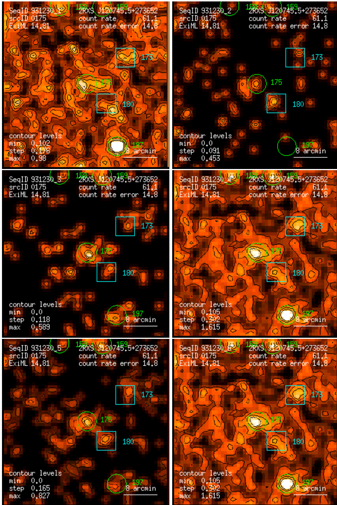
Figure 175: RASS 931230: detection 0175: band rate images, Gaussian filter: (1) PSPC channels 11 – 41, (2) 52 – 90, (3) 91 – 201, (4) 11 – 235, (5) 52 – 201, (6) 11 – 201. Broad band rates in counts/ks. Band rate contour levels in counts/ks/arcmin 2 .
