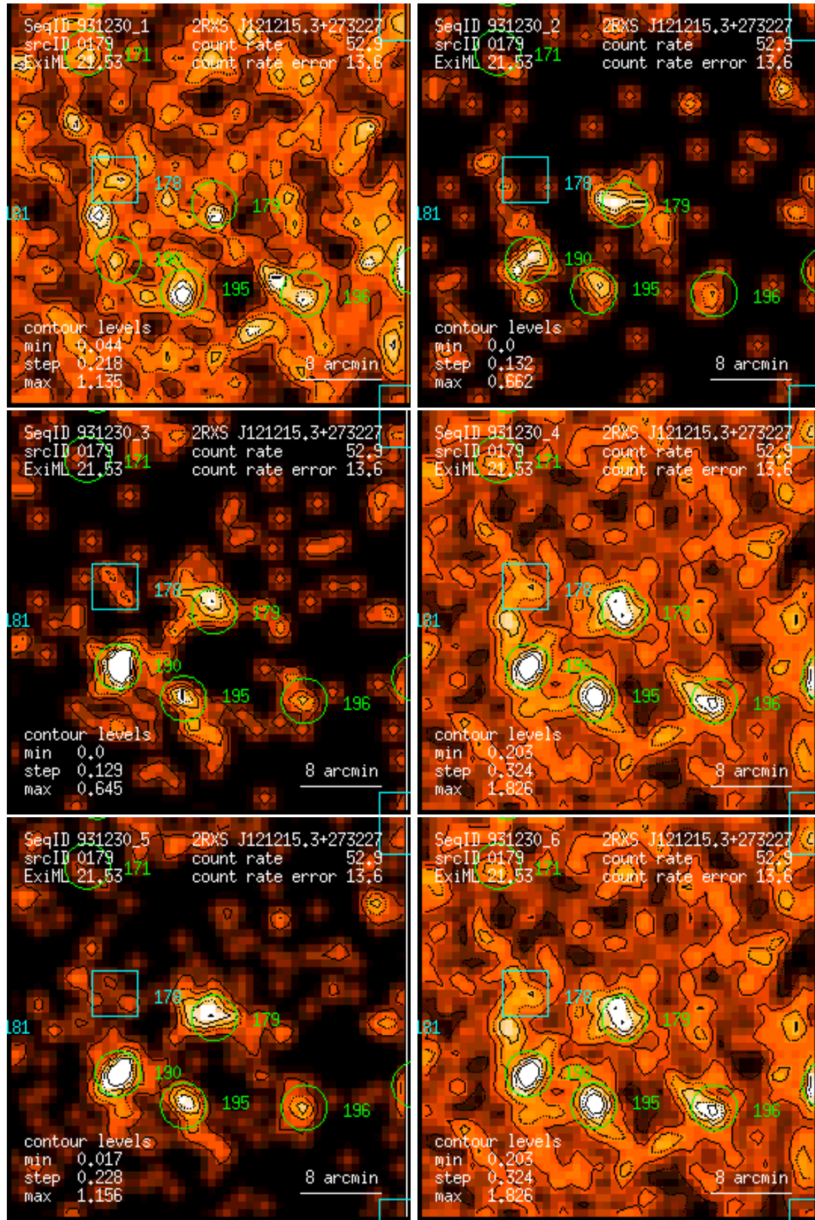
Figure 179: RASS 931230: detection 0179: band rate images, Gaussian filter: (1) PSPC channels 11 – 41, (2) 52 – 90, (3) 91 – 201, (4) 11 – 235, (5) 52 – 201, (6) 11 – 201. Broad band rates in counts/ks. Band rate contour levels in counts/ks/arcmin 2 .
