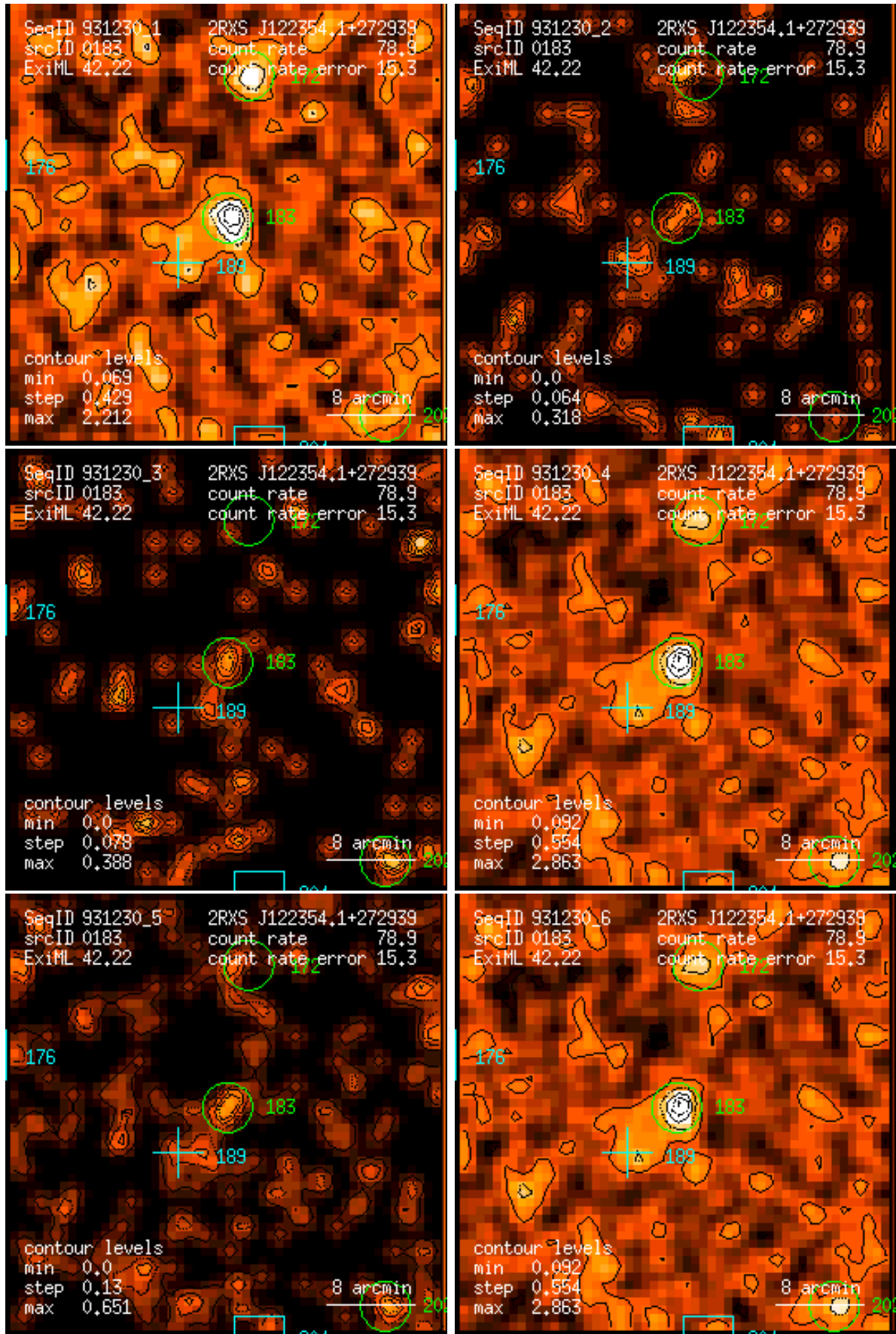
Figure 183: RASS 931230: detection 0183: band rate images, Gaussian filter: (1) PSPC channels 11 – 41, (2) 52 – 90, (3) 91 – 201, (4) 11 – 235, (5) 52 – 201, (6) 11 – 201. Broad band rates in counts/ks. Band rate contour levels in counts/ks/arcmin 2 .
