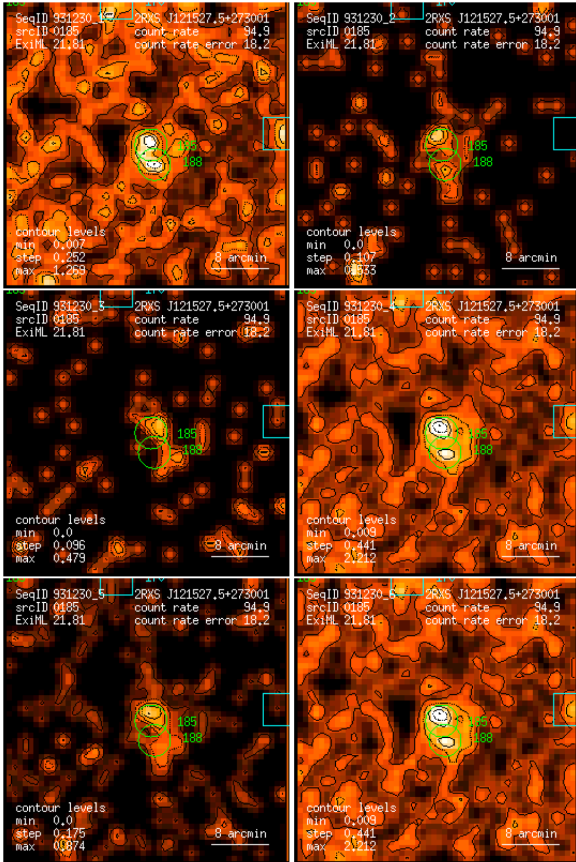
Figure 185: RASS 931230: detection 0185: band rate images, Gaussian filter: (1) PSPC channels 11 – 41, (2) 52 – 90, (3) 91 – 201, (4) 11 – 235, (5) 52 – 201, (6) 11 – 201. Broad band rates in counts/ks. Band rate contour levels in counts/ks/arcmin 2 .
