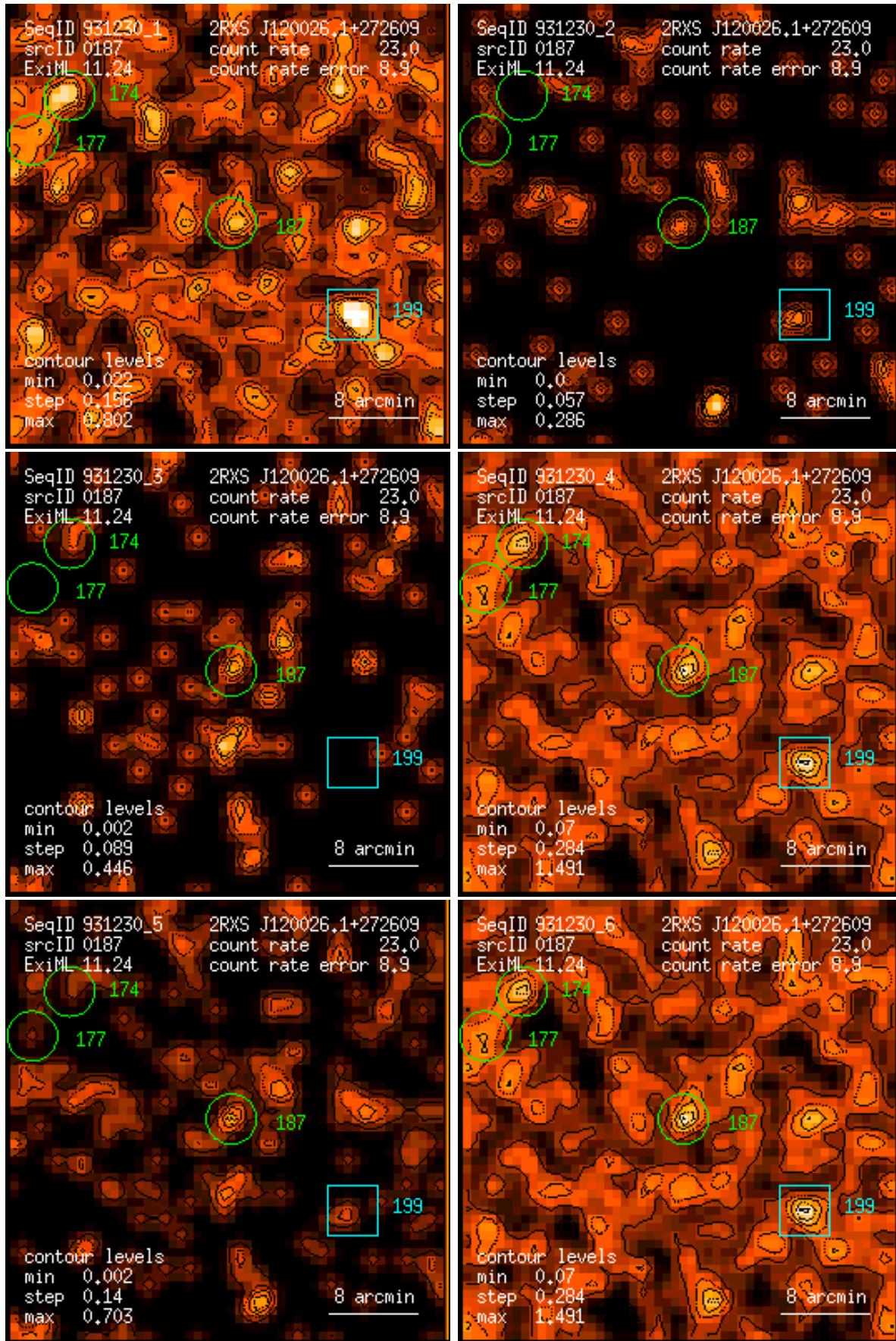
Figure 187: RASS 931230: detection 0187: band rate images, Gaussian filter: (1) PSPC channels 11 – 41, (2) 52 – 90, (3) 91 – 201, (4) 11 – 235, (5) 52 – 201, (6) 11 – 201. Broad band rates in counts/ks. Band rate contour levels in counts/ks/arcmin 2 .
