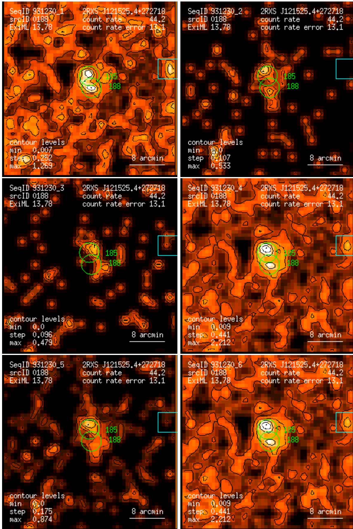
Figure 188: RASS 931230: detection 0188: band rate images, Gaussian filter: (1) PSPC channels 11 – 41, (2) 52 – 90, (3) 91 – 201, (4) 11 – 235, (5) 52 – 201, (6) 11 – 201. Broad band rates in counts/ks. Band rate contour levels in counts/ks/arcmin 2 .
