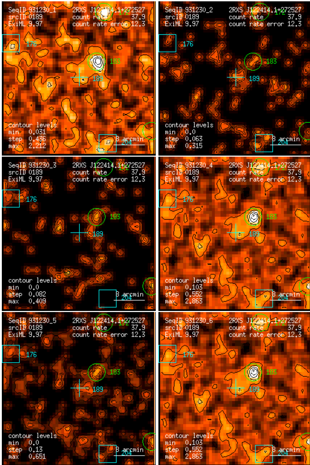
Figure 189: RASS 931230: detection 0189: band rate images, Gaussian filter: (1) PSPC channels 11 – 41, (2) 52 – 90, (3) 91 – 201, (4) 11 – 235, (5) 52 – 201, (6) 11 – 201. Broad band rates in counts/ks. Band rate contour levels in counts/ks/arcmin 2 .
