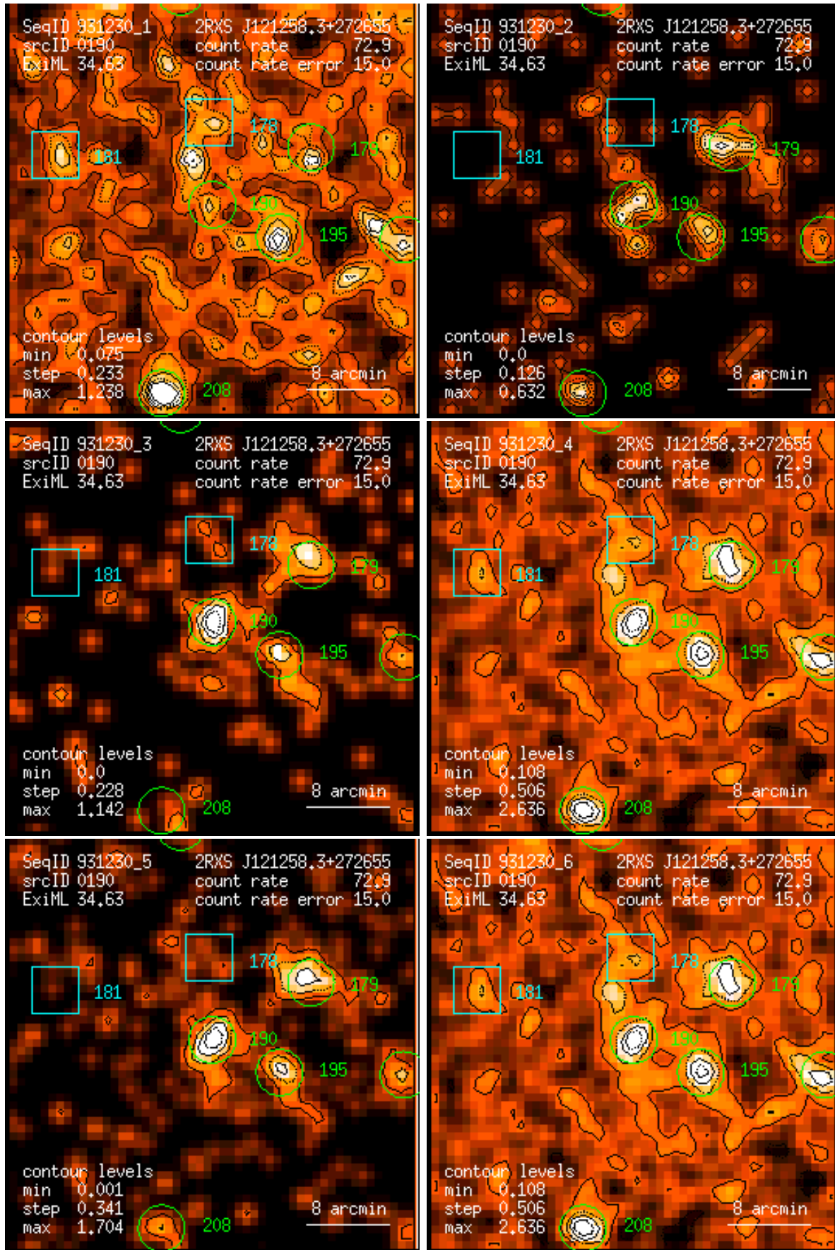
Figure 190: RASS 931230: detection 0190: band rate images, Gaussian filter: (1) PSPC channels 11 – 41, (2) 52 – 90, (3) 91 – 201, (4) 11 – 235, (5) 52 – 201, (6) 11 – 201. Broad band rates in counts/ks. Band rate contour levels in counts/ks/arcmin 2 .
