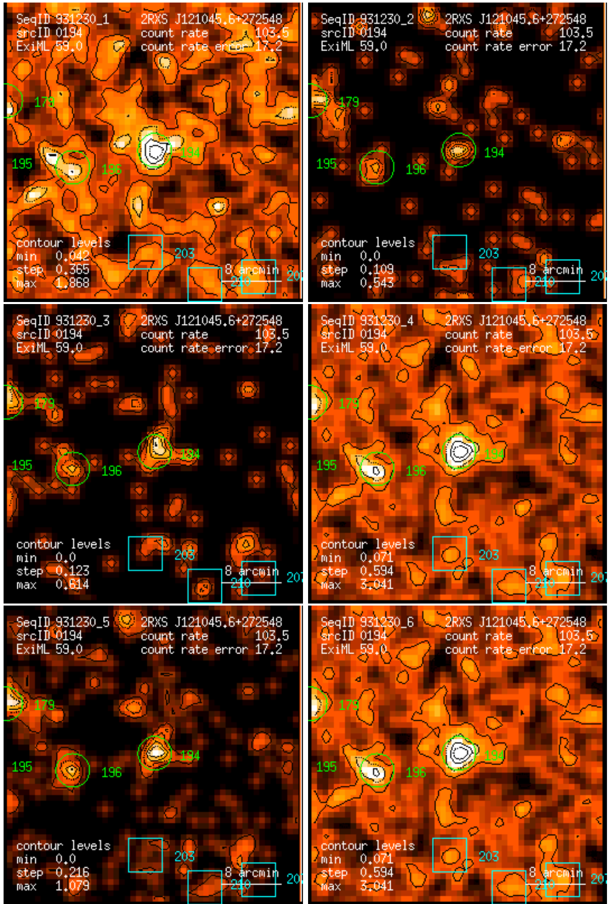
Figure 194: RASS 931230: detection 0194: band rate images, Gaussian filter: (1) PSPC channels 11 – 41, (2) 52 – 90, (3) 91 – 201, (4) 11 – 235, (5) 52 – 201, (6) 11 – 201. Broad band rates in counts/ks. Band rate contour levels in counts/ks/arcmin 2 .
