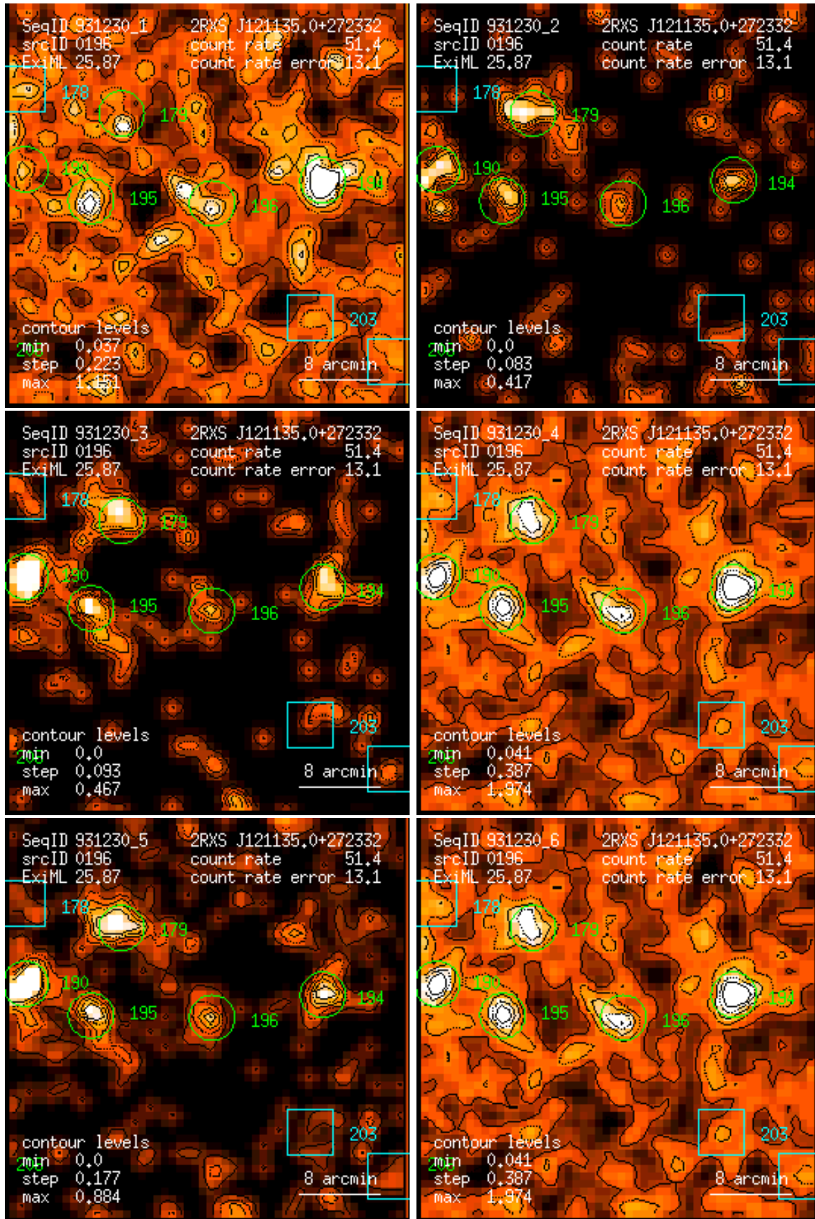
Figure 196: RASS 931230: detection 0196: band rate images, Gaussian filter: (1) PSPC channels 11 – 41, (2) 52 – 90, (3) 91 – 201, (4) 11 – 235, (5) 52 – 201, (6) 11 – 201. Broad band rates in counts/ks. Band rate contour levels in counts/ks/arcmin 2 .
