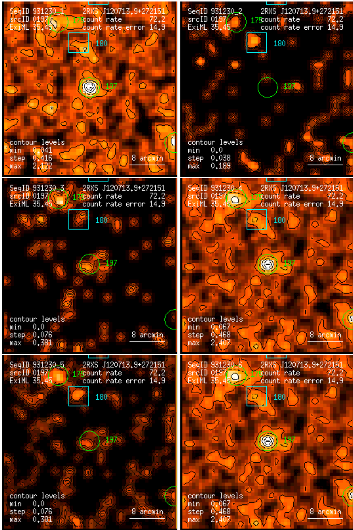
Figure 197: RASS 931230: detection 0197: band rate images, Gaussian filter: (1) PSPC channels 11 – 41, (2) 52 – 90, (3) 91 – 201, (4) 11 – 235, (5) 52 – 201, (6) 11 – 201. Broad band rates in counts/ks. Band rate contour levels in counts/ks/arcmin 2 .
