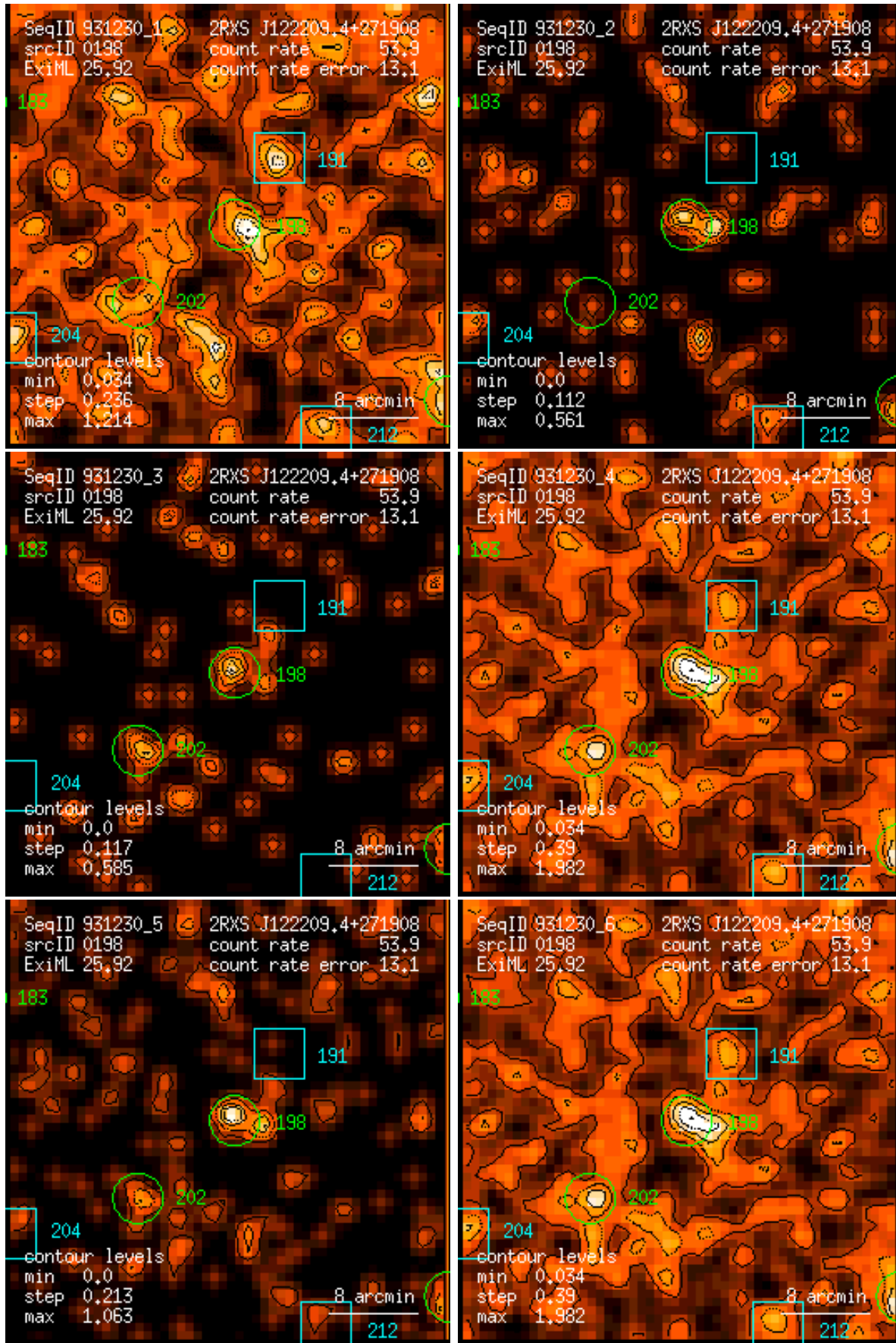
Figure 198: RASS 931230: detection 0198: band rate images, Gaussian filter: (1) PSPC channels 11 – 41, (2) 52 – 90, (3) 91 – 201, (4) 11 – 235, (5) 52 – 201, (6) 11 – 201. Broad band rates in counts/ks. Band rate contour levels in counts/ks/arcmin 2 .
