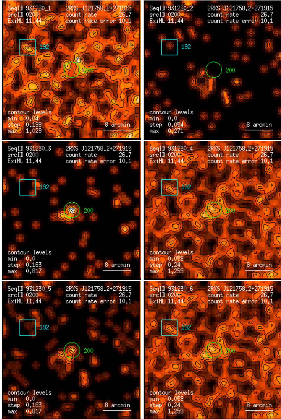
Figure 200: RASS 931230: detection 0200: band rate images, Gaussian filter: (1) PSPC channels 11 – 41, (2) 52 – 90, (3) 91 – 201, (4) 11 – 235, (5) 52 – 201, (6) 11 – 201. Broad band rates in counts/ks. Band rate contour levels in counts/ks/arcmin 2 .
