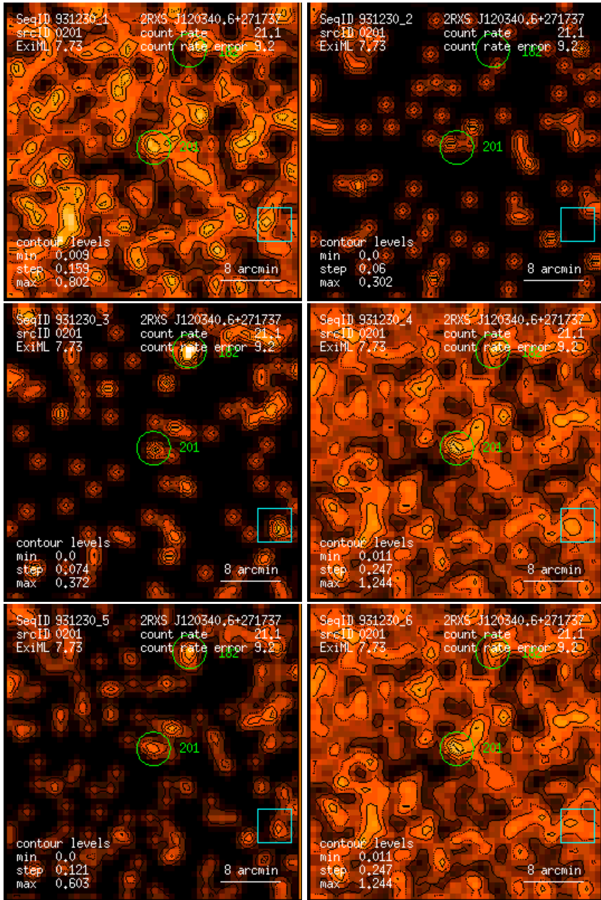
Figure 201: RASS 931230: detection 0201: band rate images, Gaussian filter: (1) PSPC channels 11 – 41, (2) 52 – 90, (3) 91 – 201, (4) 11 – 235, (5) 52 – 201, (6) 11 – 201. Broad band rates in counts/ks. Band rate contour levels in counts/ks/arcmin 2 .
