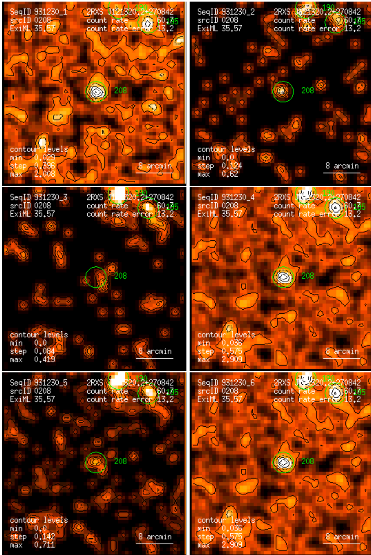
Figure 208: RASS 931230: detection 0208: band rate images, Gaussian filter: (1) PSPC channels 11 – 41, (2) 52 – 90, (3) 91 – 201, (4) 11 – 235, (5) 52 – 201, (6) 11 – 201. Broad band rates in counts/ks. Band rate contour levels in counts/ks/arcmin 2 .
