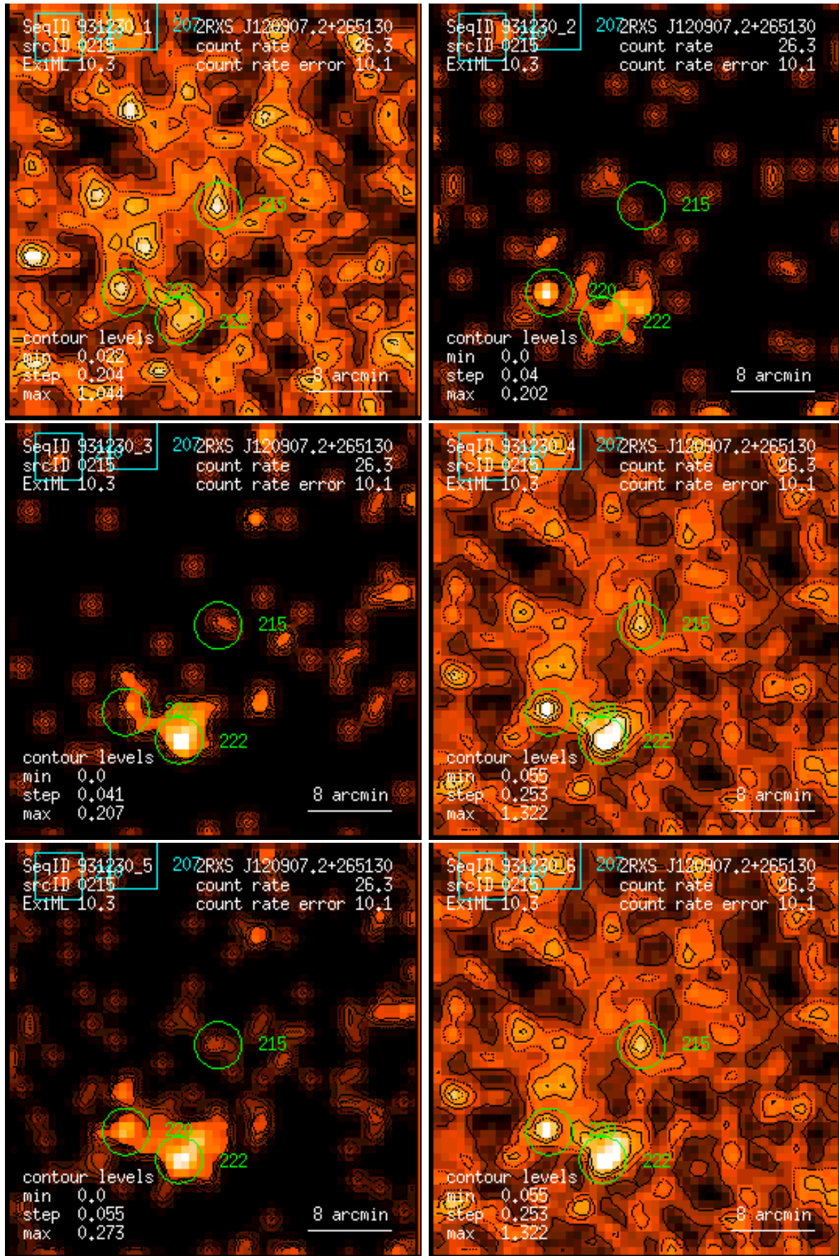
Figure 215: RASS 931230: detection 0215: band rate images, Gaussian filter: (1) PSPC channels 11 – 41, (2) 52 – 90, (3) 91 – 201, (4) 11 – 235, (5) 52 – 201, (6) 11 – 201. Broad band rates in counts/ks. Band rate contour levels in counts/ks/arcmin 2 .
