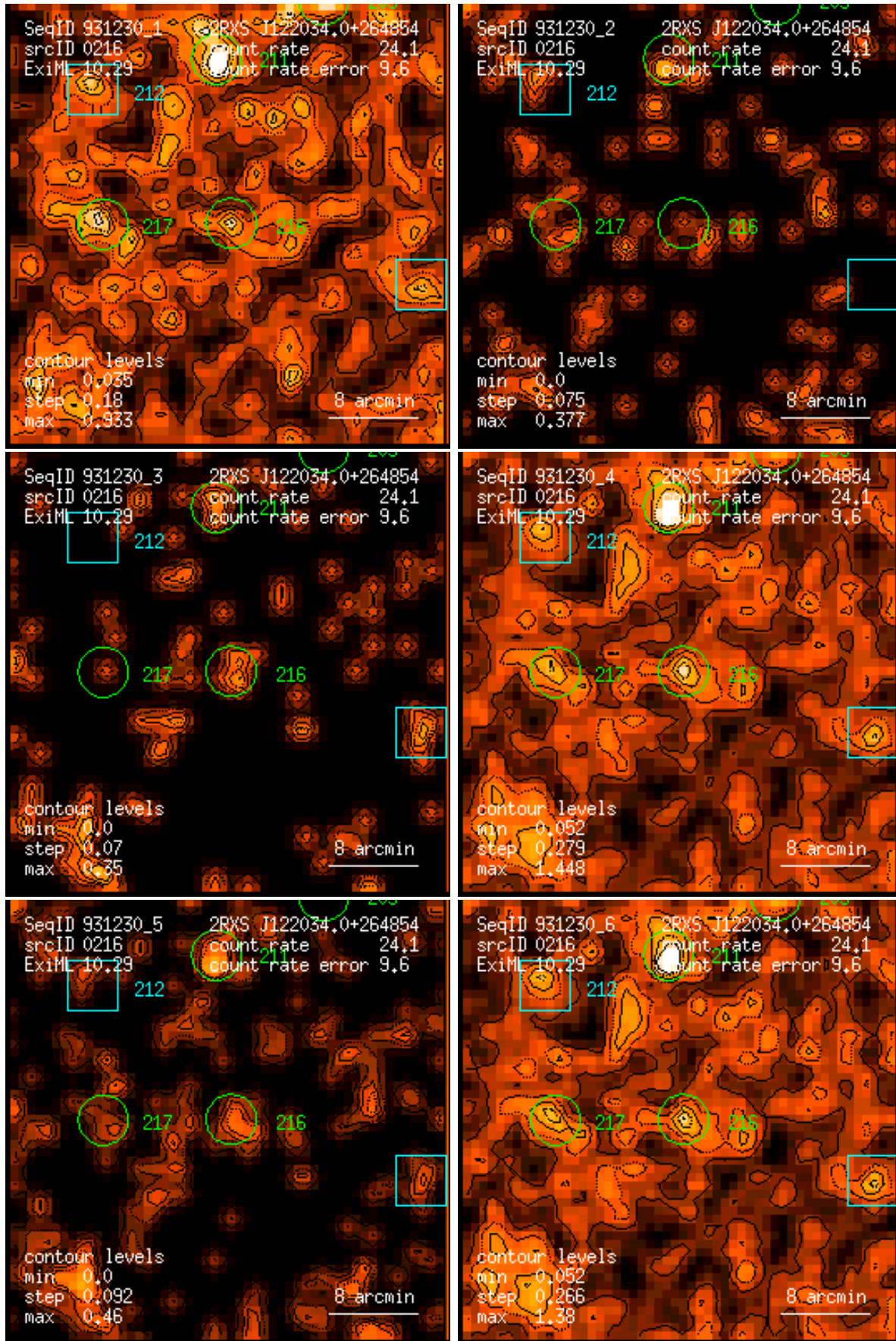
Figure 216: RASS 931230: detection 0216: band rate images, Gaussian filter: (1) PSPC channels 11 – 41, (2) 52 – 90, (3) 91 – 201, (4) 11 – 235, (5) 52 – 201, (6) 11 – 201. Broad band rates in counts/ks. Band rate contour levels in counts/ks/arcmin 2 .
