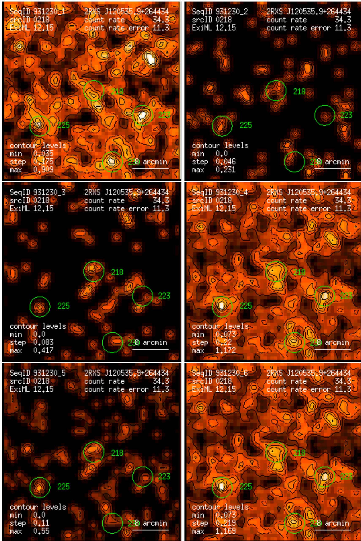
Figure 218: RASS 931230: detection 0218: band rate images, Gaussian filter: (1) PSPC channels 11 – 41, (2) 52 – 90, (3) 91 – 201, (4) 11 – 235, (5) 52 – 201, (6) 11 – 201. Broad band rates in counts/ks. Band rate contour levels in counts/ks/arcmin 2 .
