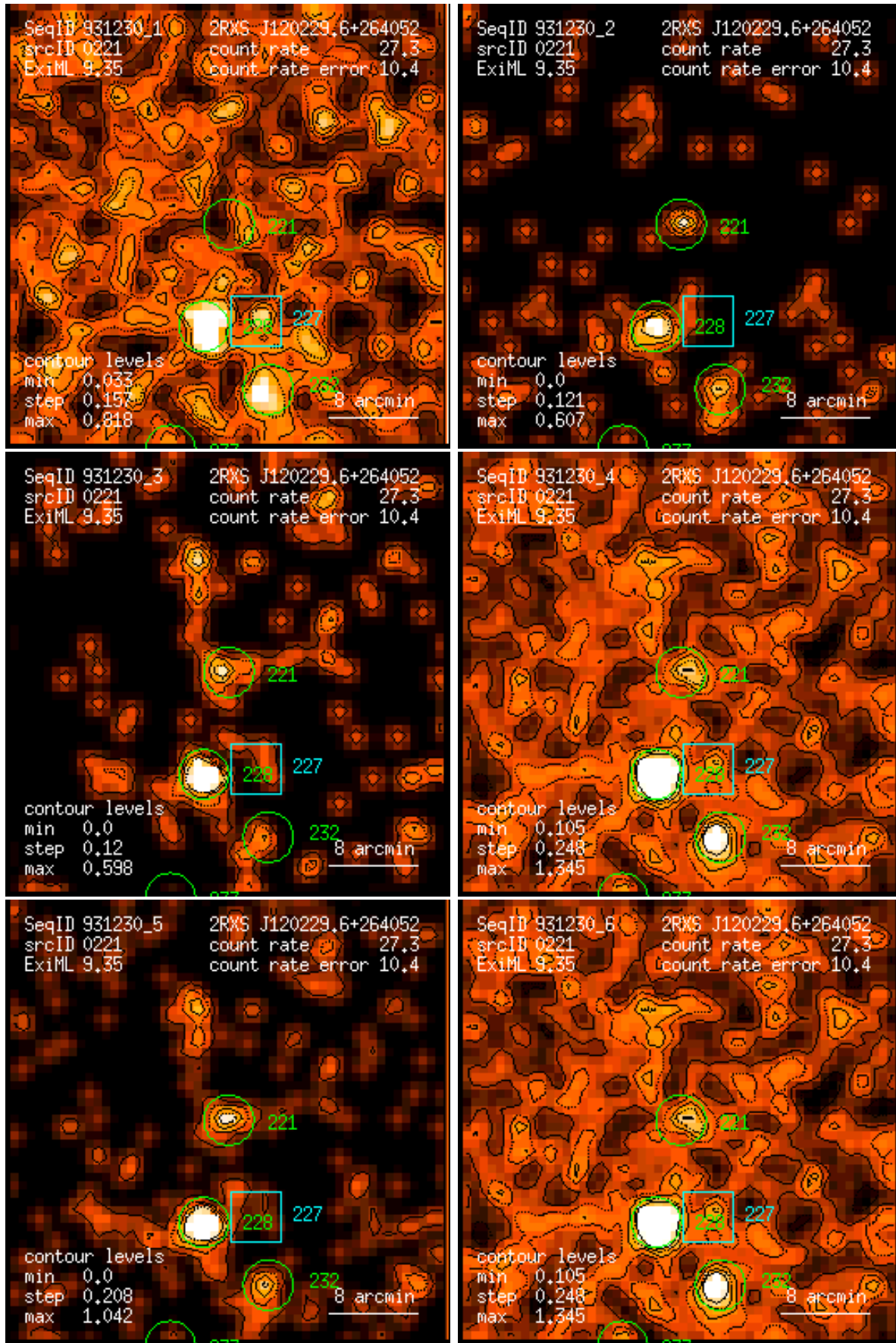
Figure 221: RASS 931230: detection 0221: band rate images, Gaussian filter: (1) PSPC channels 11 – 41, (2) 52 – 90, (3) 91 – 201, (4) 11 – 235, (5) 52 – 201, (6) 11 – 201. Broad band rates in counts/ks. Band rate contour levels in counts/ks/arcmin 2 .
