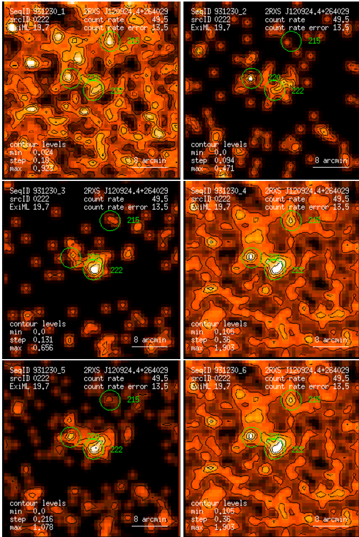
Figure 222: RASS 931230: detection 0222: band rate images, Gaussian filter: (1) PSPC channels 11 – 41, (2) 52 – 90, (3) 91 – 201, (4) 11 – 235, (5) 52 – 201, (6) 11 – 201. Broad band rates in counts/ks. Band rate contour levels in counts/ks/arcmin 2 .
