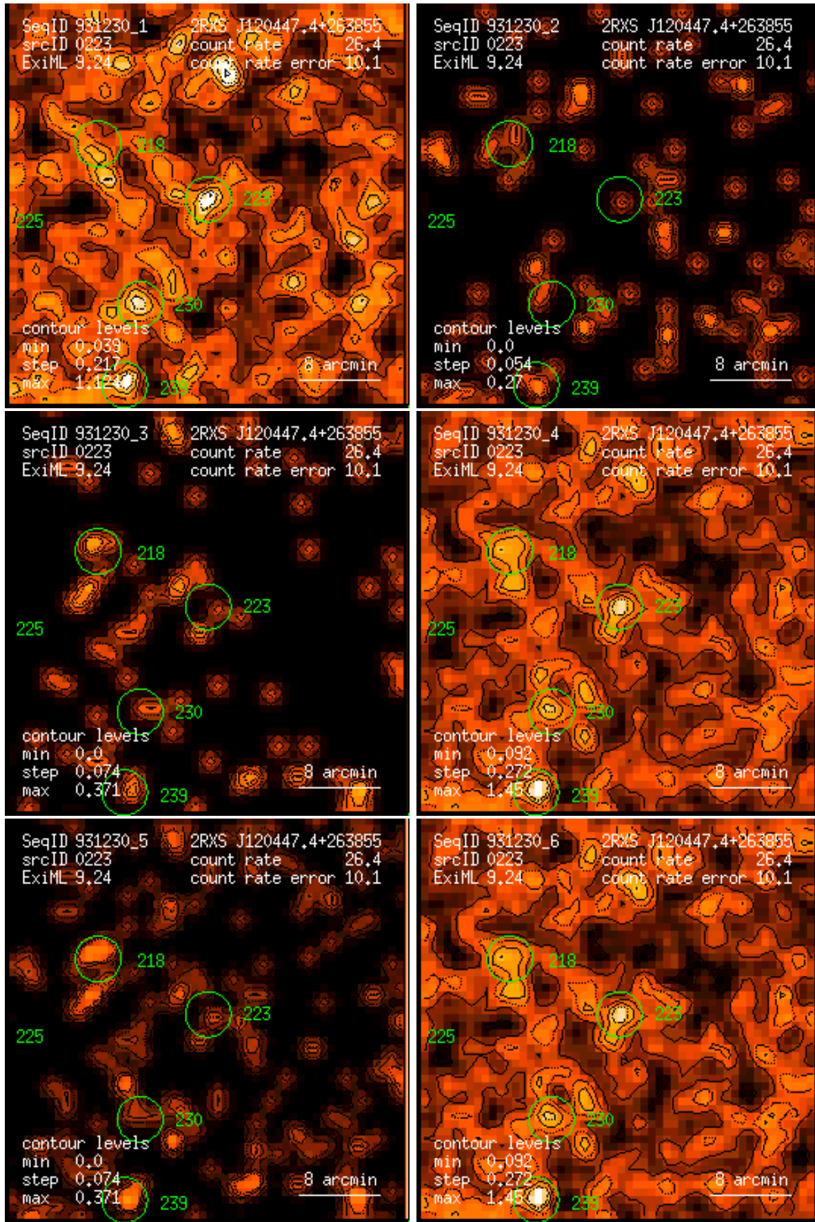
Figure 223: RASS 931230: detection 0223: band rate images, Gaussian filter: (1) PSPC channels 11 – 41, (2) 52 – 90, (3) 91 – 201, (4) 11 – 235, (5) 52 – 201, (6) 11 – 201. Broad band rates in counts/ks. Band rate contour levels in counts/ks/arcmin 2 .
