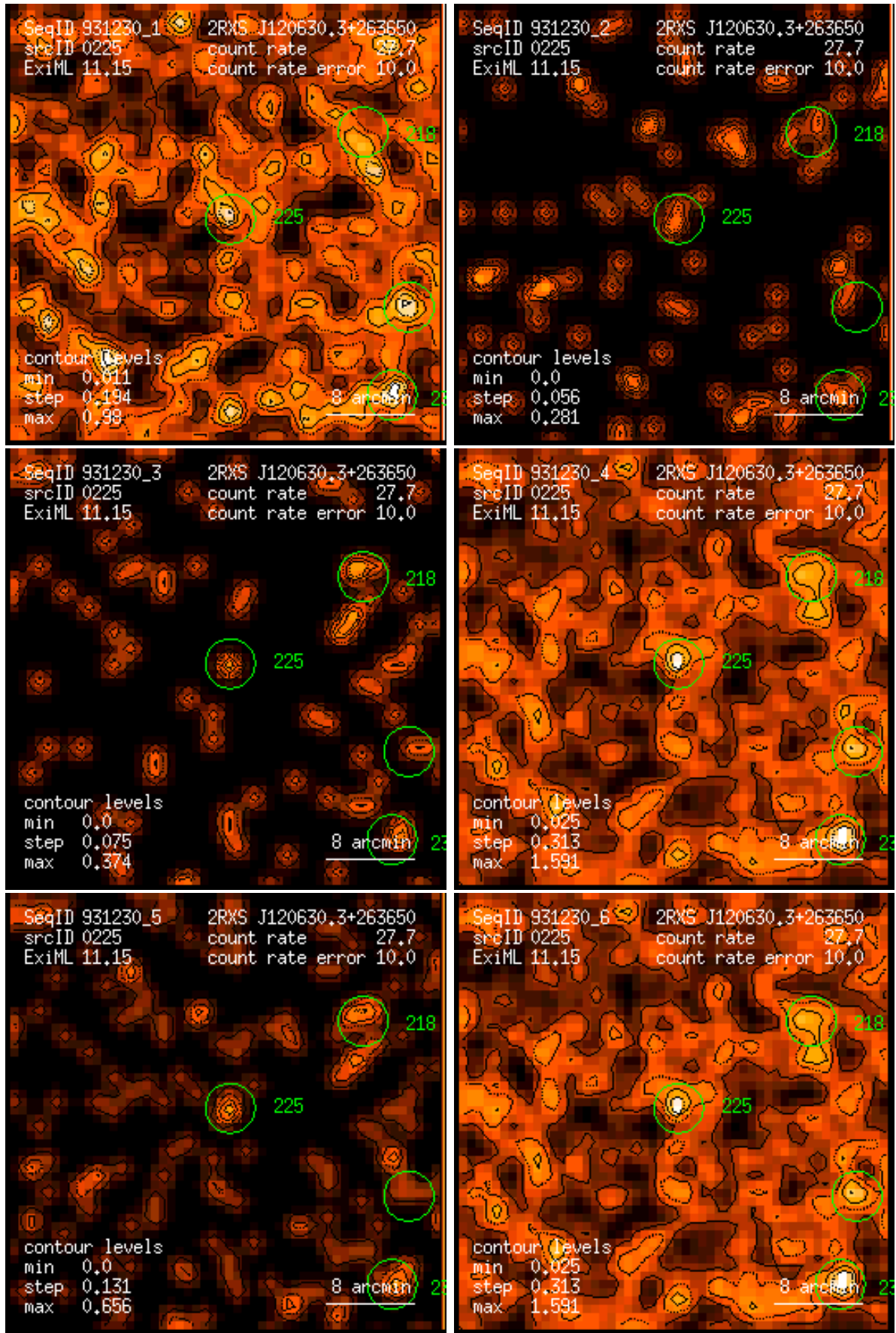
Figure 225: RASS 931230: detection 0225: band rate images, Gaussian filter: (1) PSPC channels 11 – 41, (2) 52 – 90, (3) 91 – 201, (4) 11 – 235, (5) 52 – 201, (6) 11 – 201. Broad band rates in counts/ks. Band rate contour levels in counts/ks/arcmin 2 .
