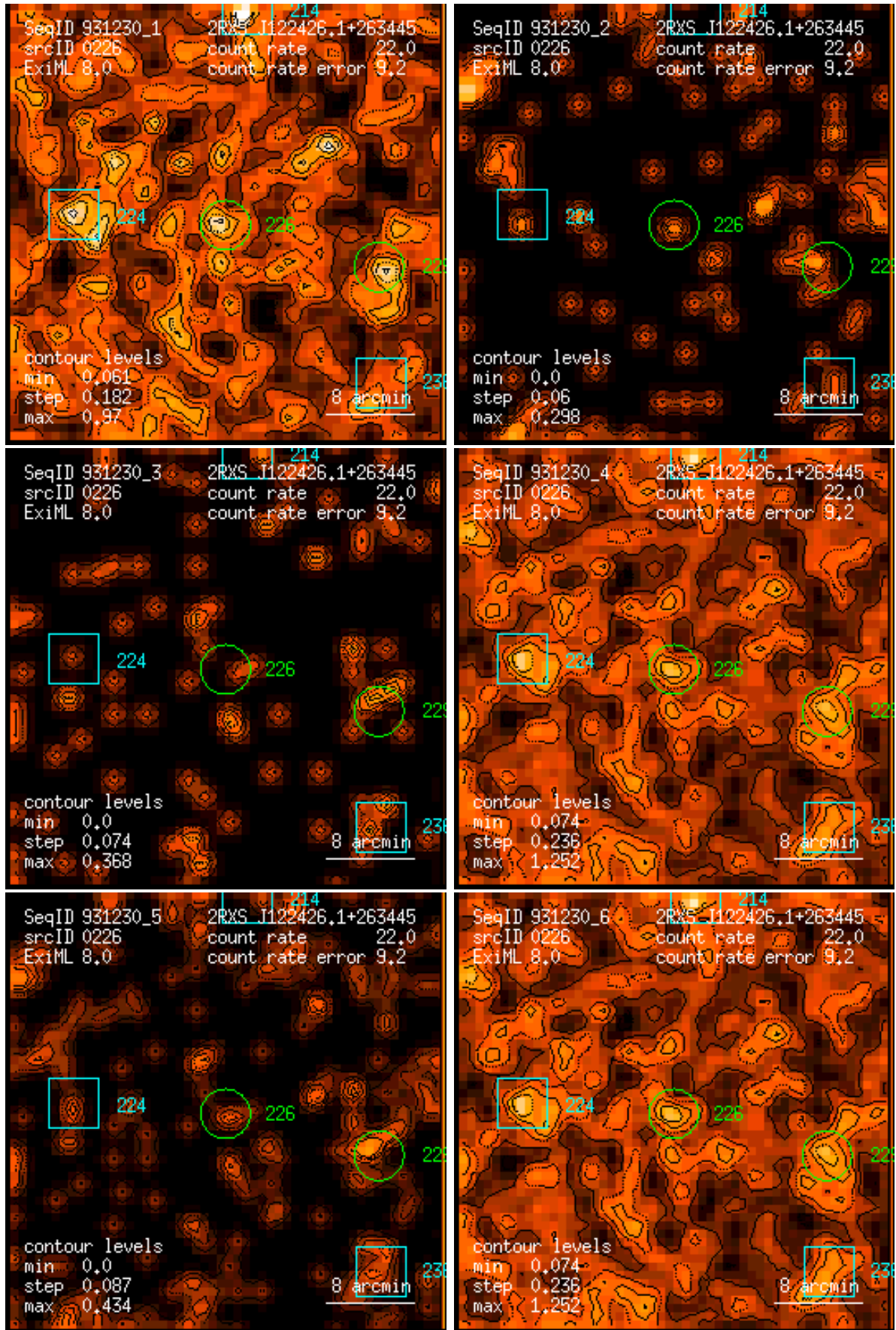
Figure 226: RASS 931230: detection 0226: band rate images, Gaussian filter: (1) PSPC channels 11 – 41, (2) 52 – 90, (3) 91 – 201, (4) 11 – 235, (5) 52 – 201, (6) 11 – 201. Broad band rates in counts/ks. Band rate contour levels in counts/ks/arcmin 2 .
