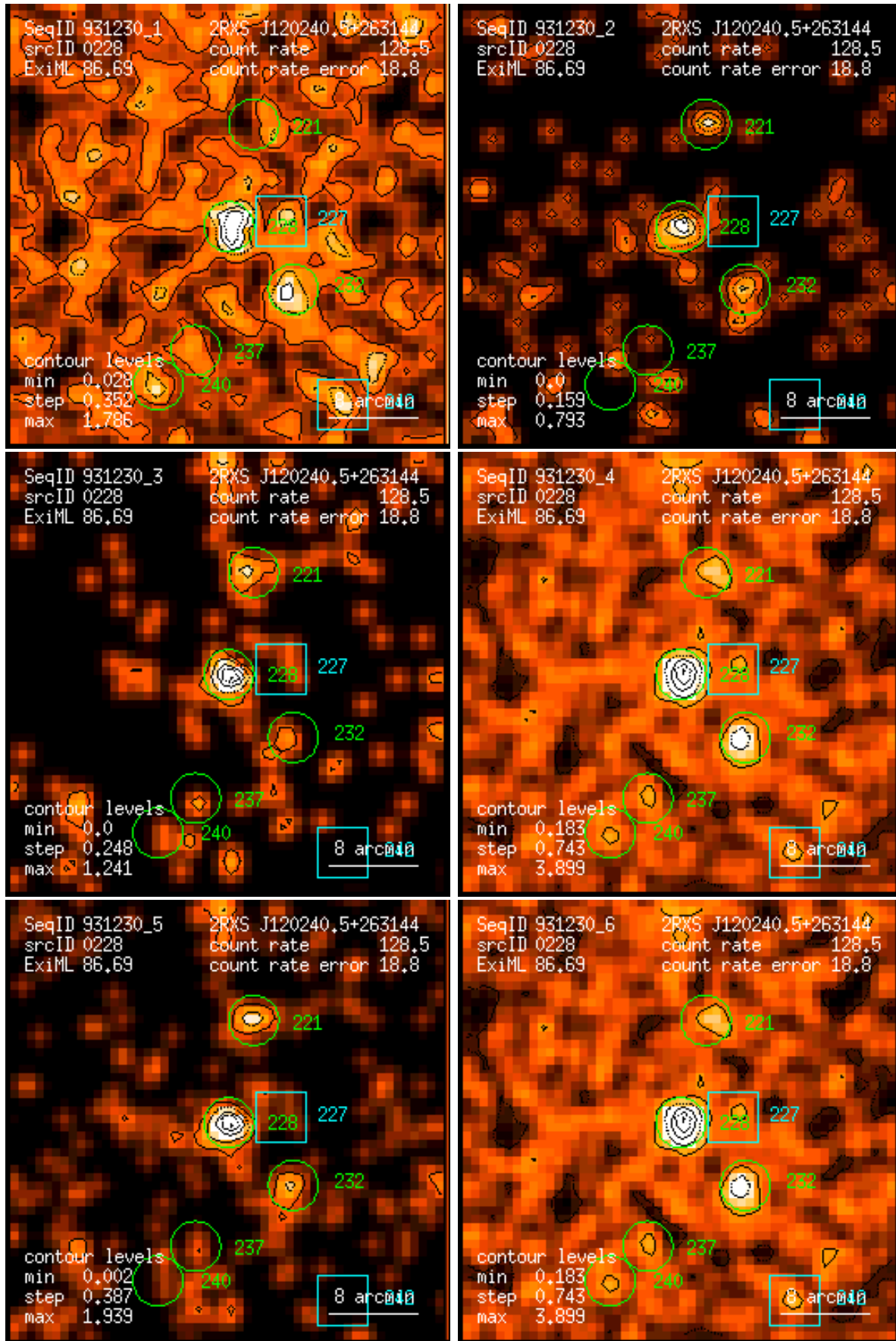
Figure 228: RASS 931230: detection 0228: band rate images, Gaussian filter: (1) PSPC channels 11 – 41, (2) 52 – 90, (3) 91 – 201, (4) 11 – 235, (5) 52 – 201, (6) 11 – 201. Broad band rates in counts/ks. Band rate contour levels in counts/ks/arcmin 2 .
