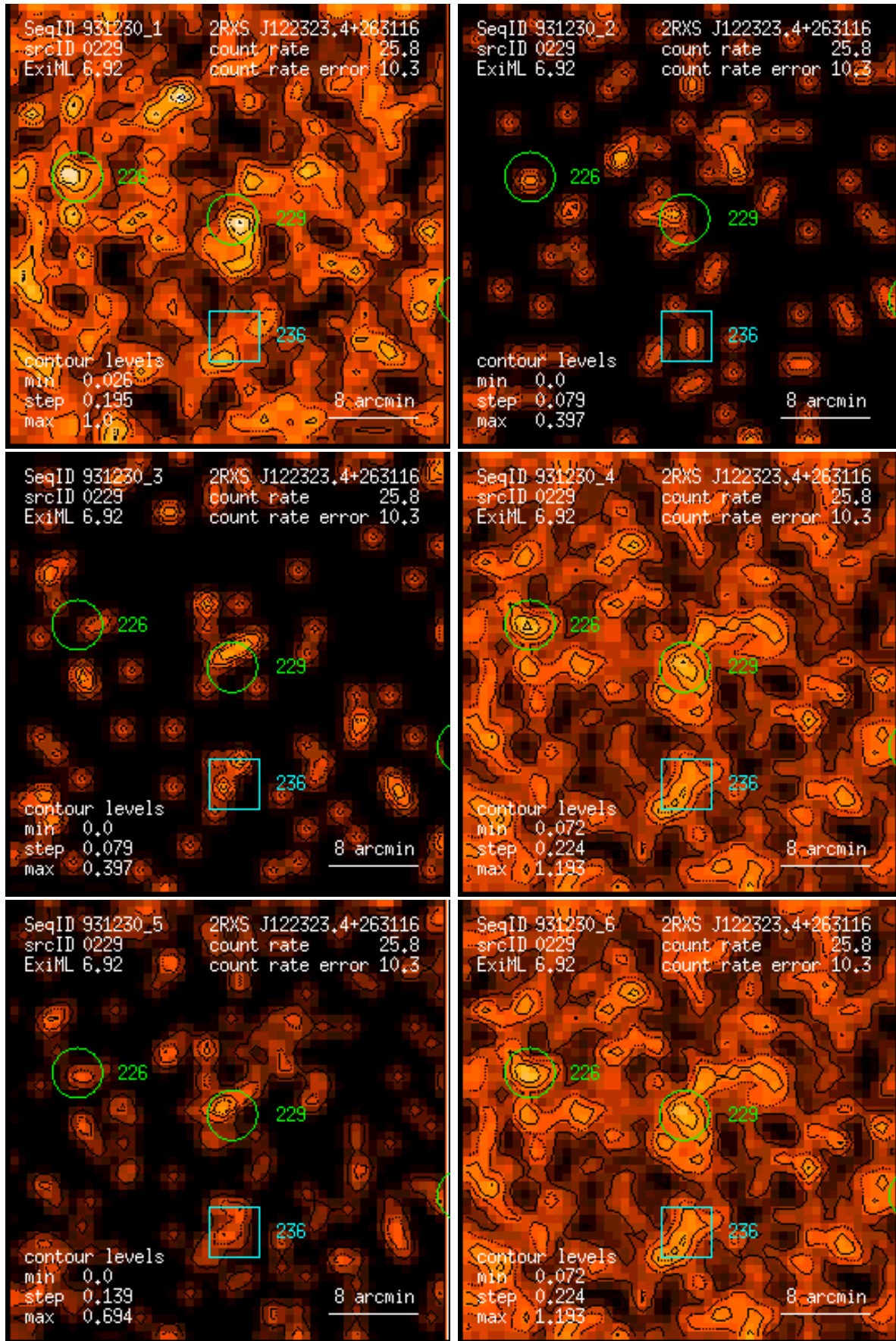
Figure 229: RASS 931230: detection 0229: band rate images, Gaussian filter: (1) PSPC channels 11 – 41, (2) 52 – 90, (3) 91 – 201, (4) 11 – 235, (5) 52 – 201, (6) 11 – 201. Broad band rates in counts/ks. Band rate contour levels in counts/ks/arcmin 2 .
