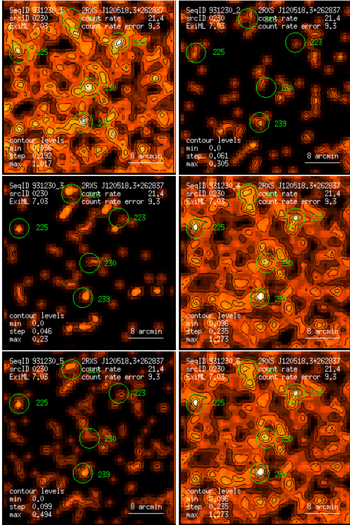
Figure 230: RASS 931230: detection 0230: band rate images, Gaussian filter: (1) PSPC channels 11 – 41, (2) 52 – 90, (3) 91 – 201, (4) 11 – 235, (5) 52 – 201, (6) 11 – 201. Broad band rates in counts/ks. Band rate contour levels in counts/ks/arcmin 2 .
