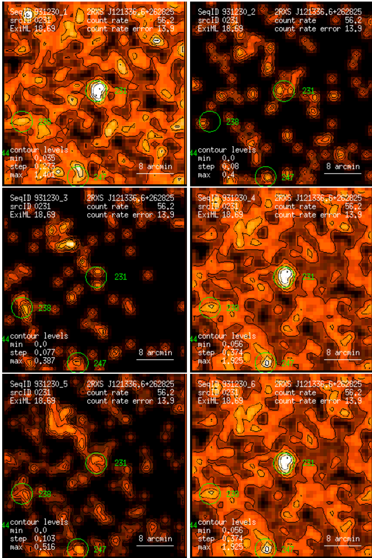
Figure 231: RASS 931230: detection 0231: band rate images, Gaussian filter: (1) PSPC channels 11 – 41, (2) 52 – 90, (3) 91 – 201, (4) 11 – 235, (5) 52 – 201, (6) 11 – 201. Broad band rates in counts/ks. Band rate contour levels in counts/ks/arcmin 2 .
