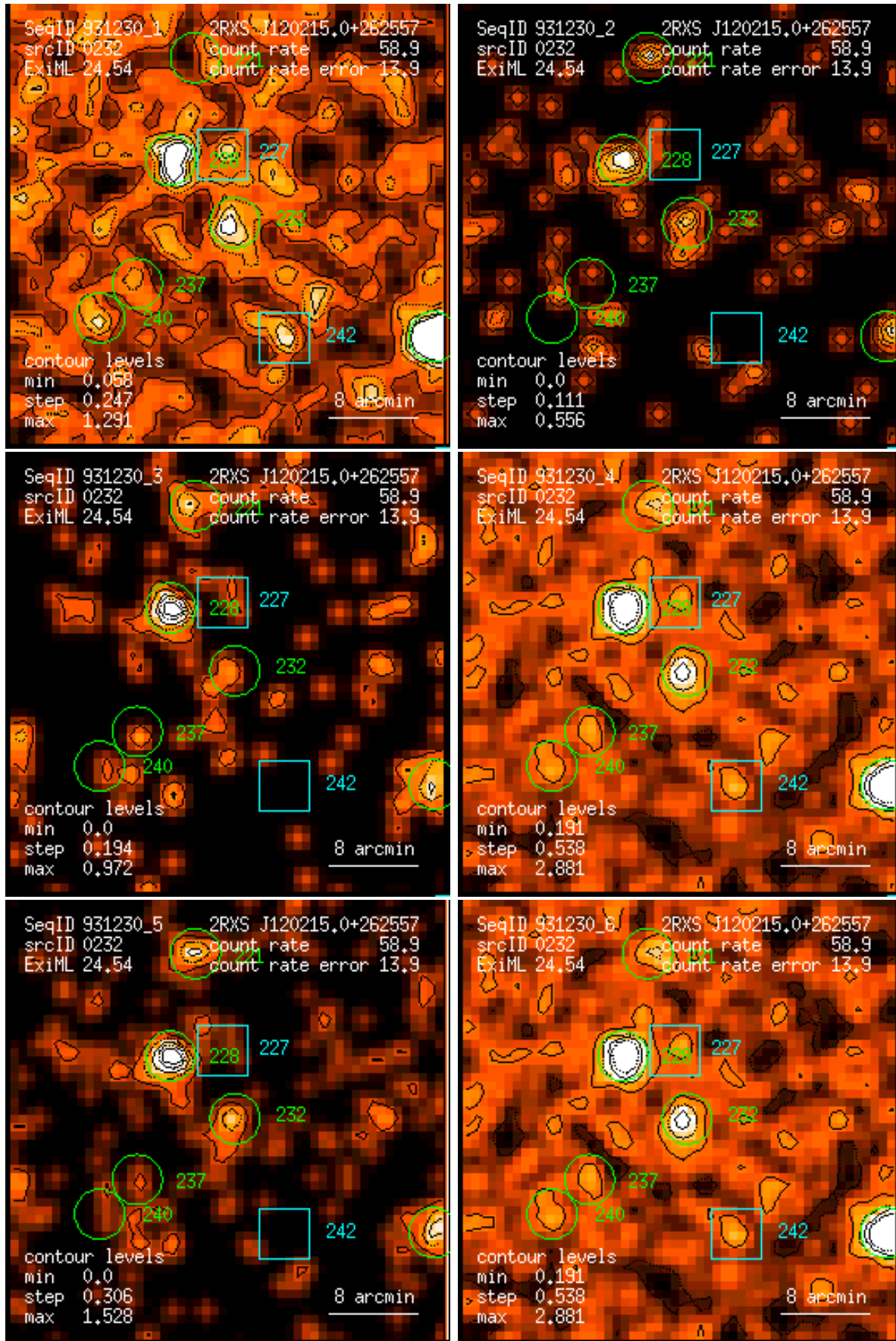
Figure 232: RASS 931230: detection 0232: band rate images, Gaussian filter: (1) PSPC channels 11 – 41, (2) 52 – 90, (3) 91 – 201, (4) 11 – 235, (5) 52 – 201, (6) 11 – 201. Broad band rates in counts/ks. Band rate contour levels in counts/ks/arcmin 2 .
