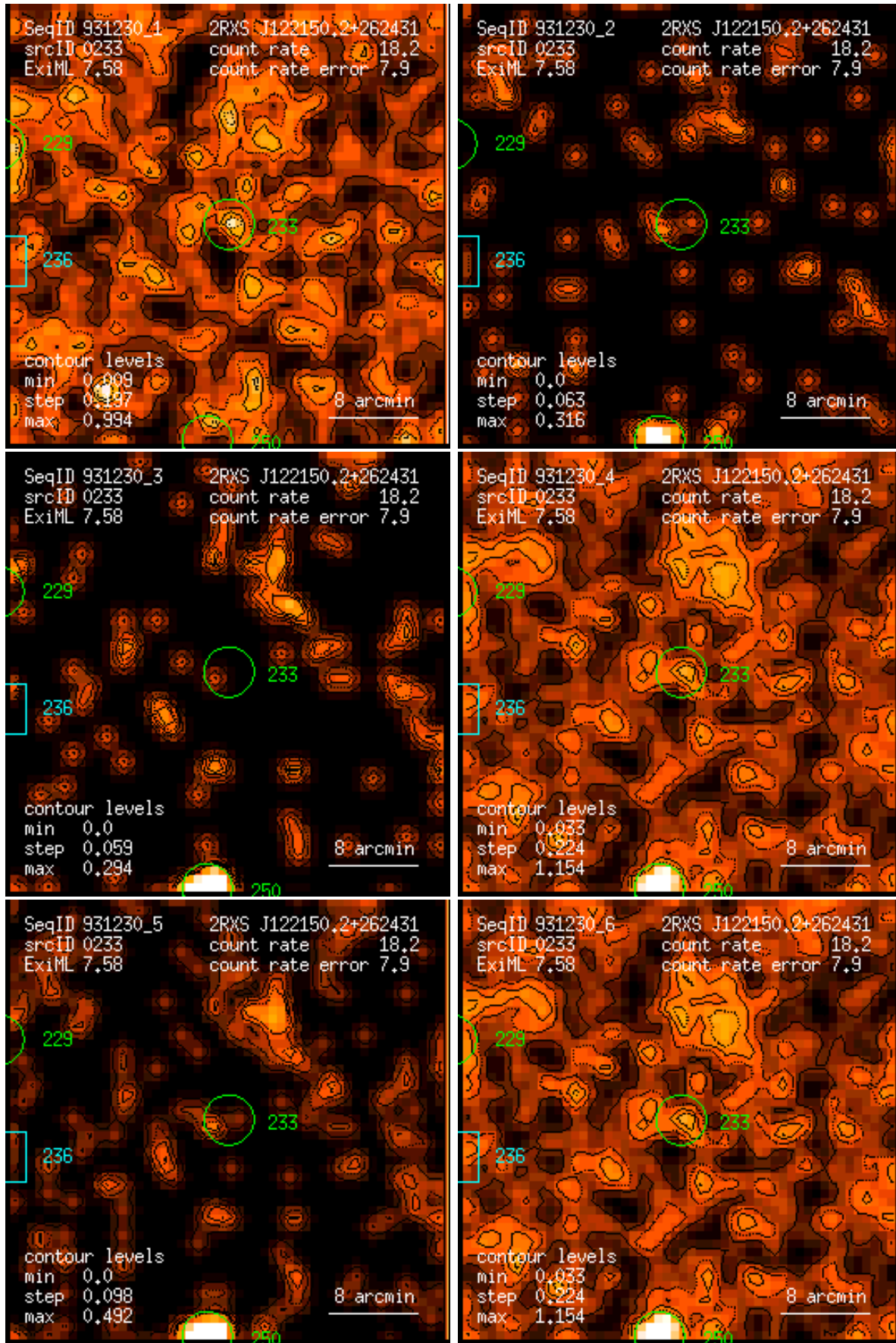
Figure 233: RASS 931230: detection 0233: band rate images, Gaussian filter: (1) PSPC channels 11 – 41, (2) 52 – 90, (3) 91 – 201, (4) 11 – 235, (5) 52 – 201, (6) 11 – 201. Broad band rates in counts/ks. Band rate contour levels in counts/ks/arcmin 2 .
