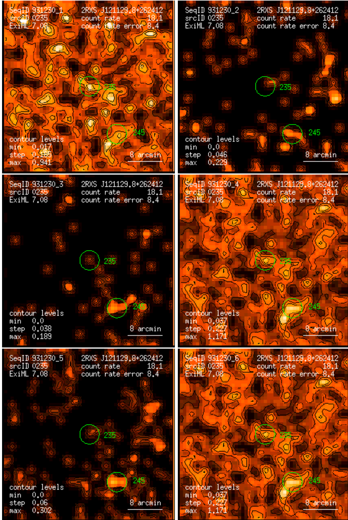
Figure 235: RASS 931230: detection 0235: band rate images, Gaussian filter: (1) PSPC channels 11 – 41, (2) 52 – 90, (3) 91 – 201, (4) 11 – 235, (5) 52 – 201, (6) 11 – 201. Broad band rates in counts/ks. Band rate contour levels in counts/ks/arcmin 2 .
