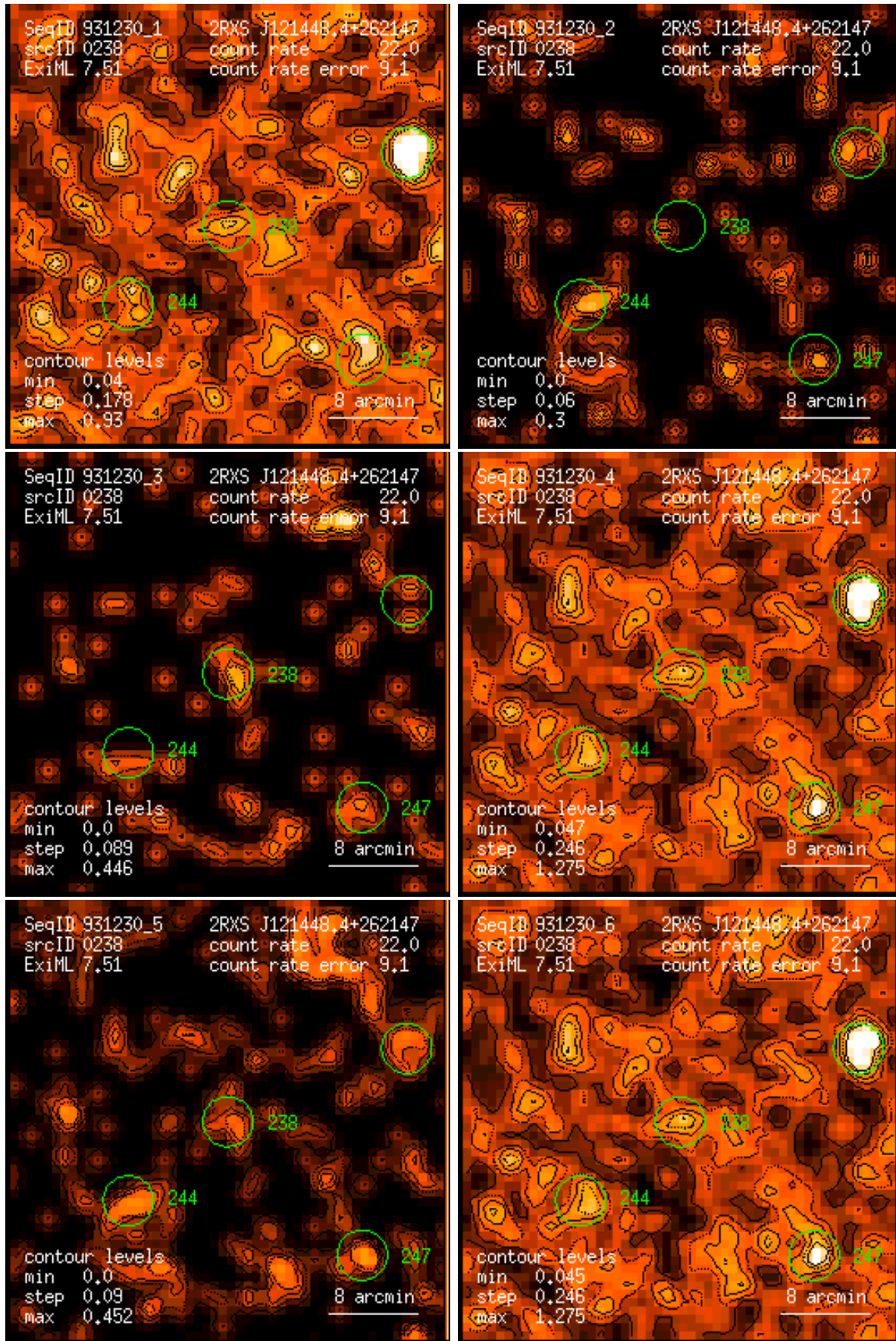
Figure 238: RASS 931230: detection 0238: band rate images, Gaussian filter: (1) PSPC channels 11 – 41, (2) 52 – 90, (3) 91 – 201, (4) 11 – 235, (5) 52 – 201, (6) 11 – 201. Broad band rates in counts/ks. Band rate contour levels in counts/ks/arcmin 2 .
