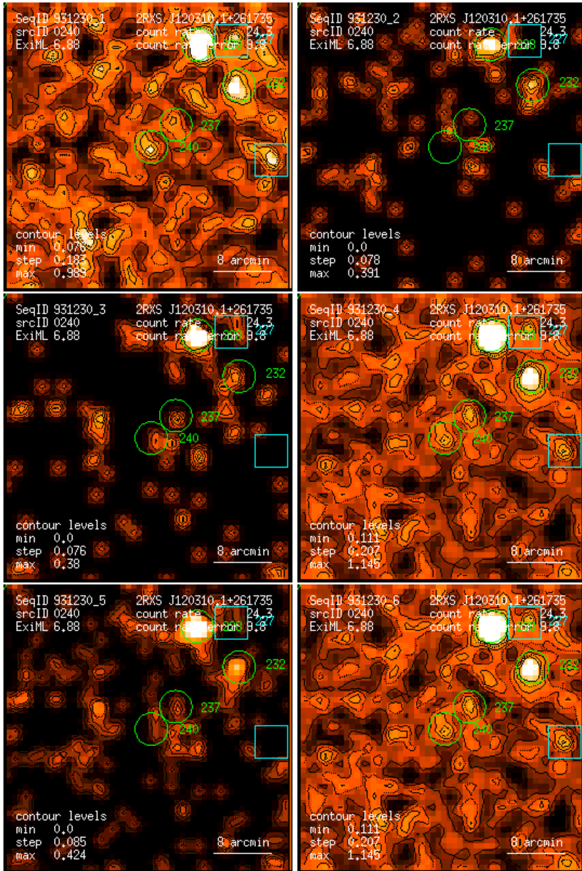
Figure 240: RASS 931230: detection 0240: band rate images, Gaussian filter: (1) PSPC channels 11 – 41, (2) 52 – 90, (3) 91 – 201, (4) 11 – 235, (5) 52 – 201, (6) 11 – 201. Broad band rates in counts/ks. Band rate contour levels in counts/ks/arcmin 2 .
