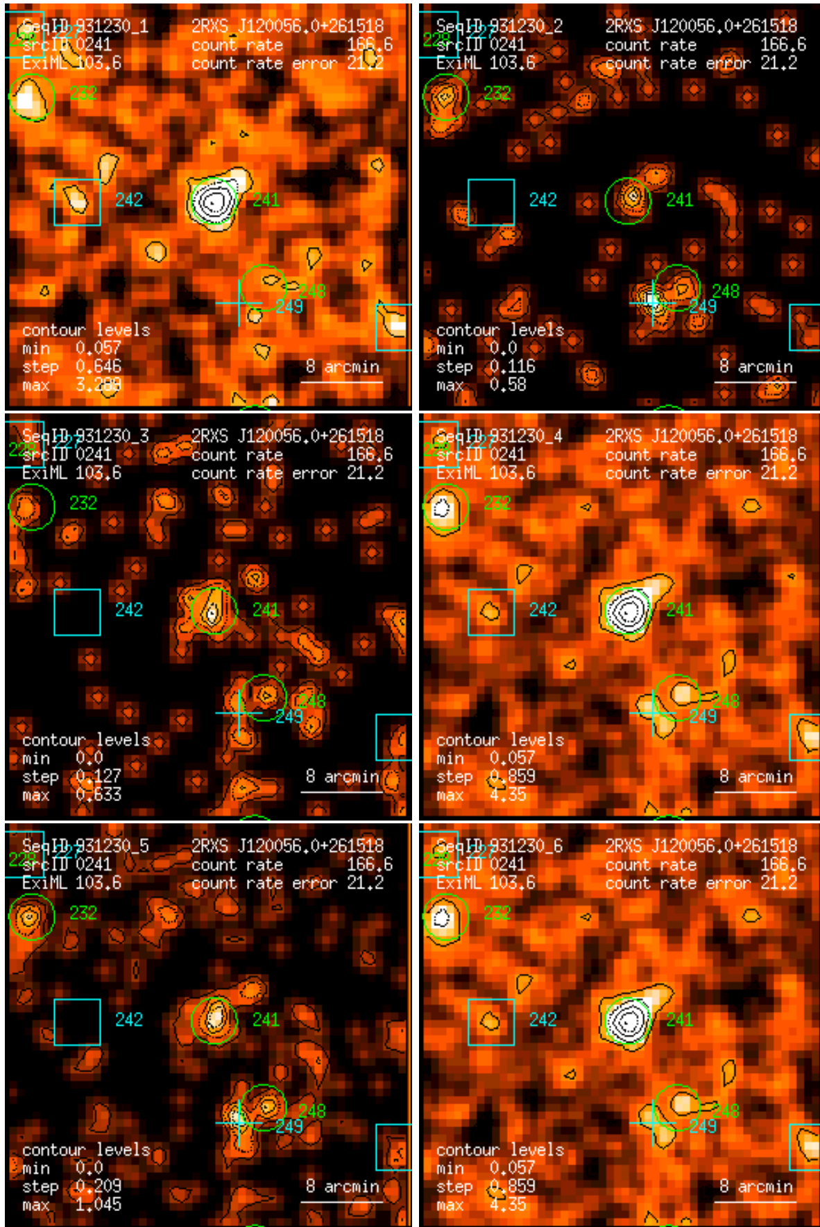
Figure 241: RASS 931230: detection 0241: band rate images, Gaussian filter: (1) PSPC channels 11 – 41, (2) 52 – 90, (3) 91 – 201, (4) 11 – 235, (5) 52 – 201, (6) 11 – 201. Broad band rates in counts/ks. Band rate contour levels in counts/ks/arcmin 2 .
