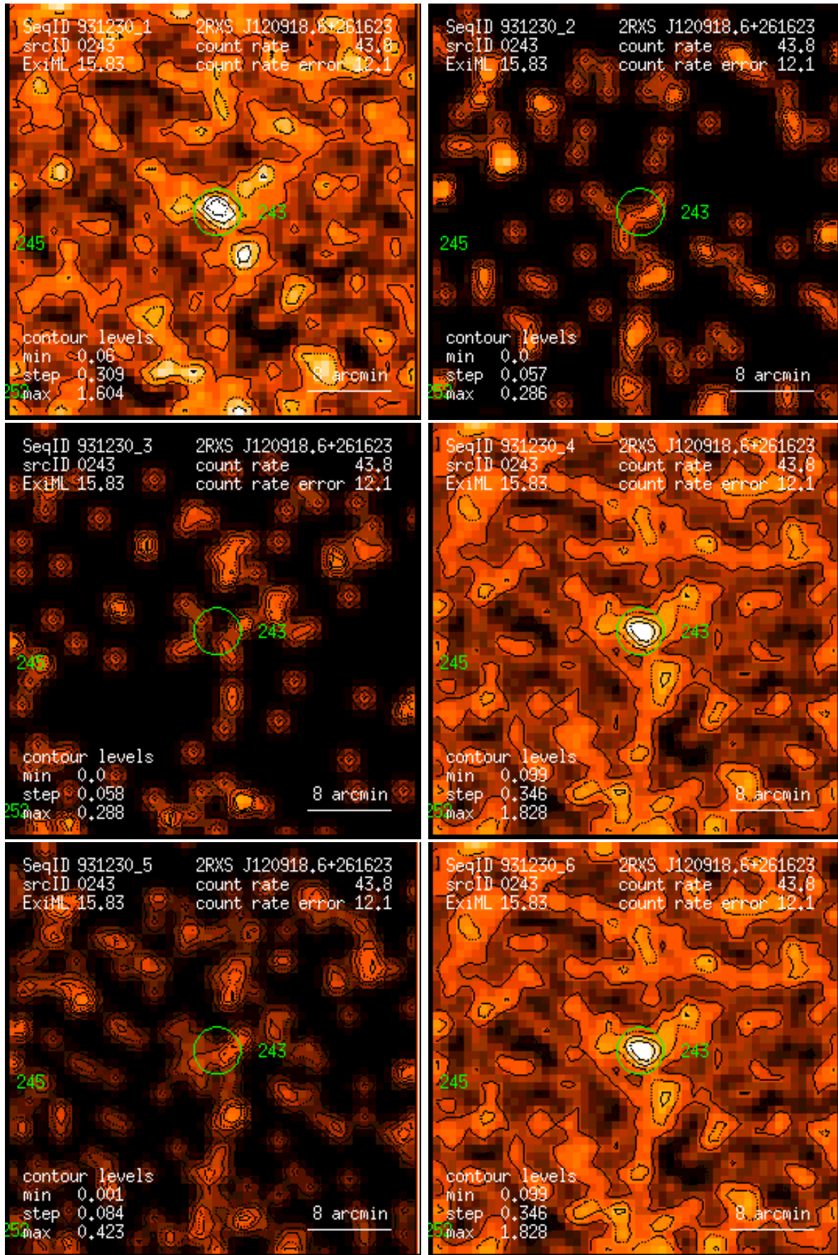
Figure 243: RASS 931230: detection 0243: band rate images, Gaussian filter: (1) PSPC channels 11 – 41, (2) 52 – 90, (3) 91 – 201, (4) 11 – 235, (5) 52 – 201, (6) 11 – 201. Broad band rates in counts/ks. Band rate contour levels in counts/ks/arcmin 2 .
