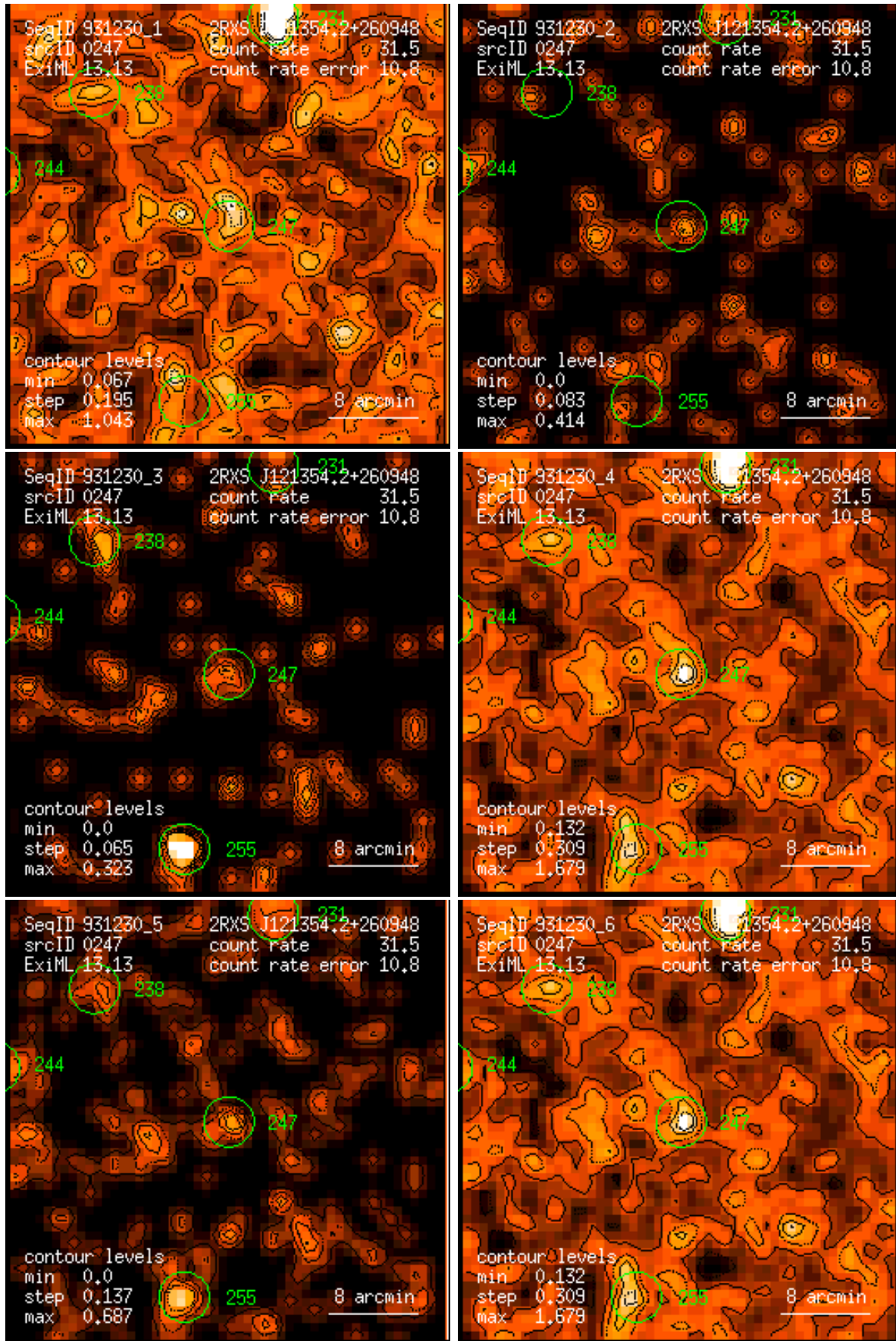
Figure 247: RASS 931230: detection 0247: band rate images, Gaussian filter: (1) PSPC channels 11 – 41, (2) 52 – 90, (3) 91 – 201, (4) 11 – 235, (5) 52 – 201, (6) 11 – 201. Broad band rates in counts/ks. Band rate contour levels in counts/ks/arcmin 2 .
