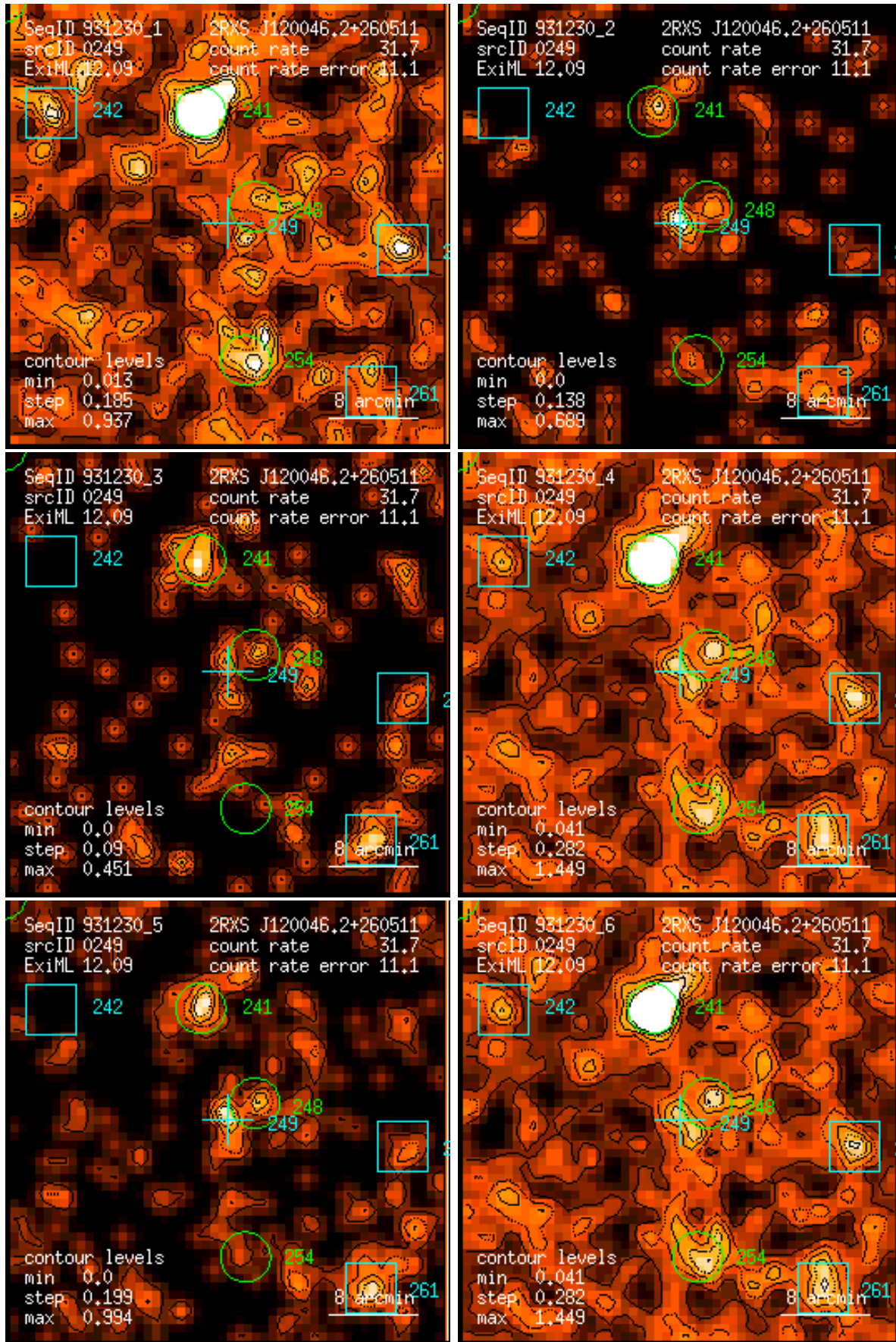
Figure 249: RASS 931230: detection 0249: band rate images, Gaussian filter: (1) PSPC channels 11 – 41, (2) 52 – 90, (3) 91 – 201, (4) 11 – 235, (5) 52 – 201, (6) 11 – 201. Broad band rates in counts/ks. Band rate contour levels in counts/ks/arcmin 2 .
