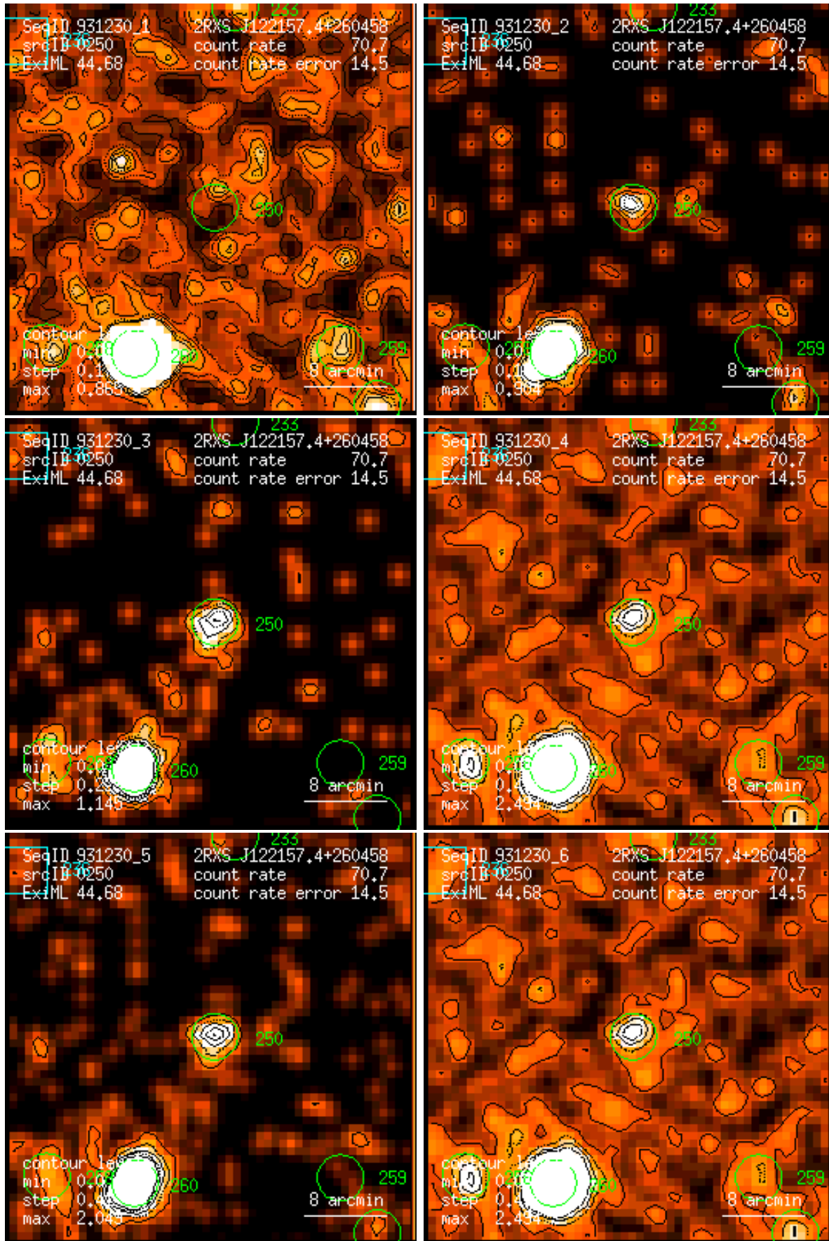
Figure 250: RASS 931230: detection 0250: band rate images, Gaussian filter: (1) PSPC channels 11 – 41, (2) 52 – 90, (3) 91 – 201, (4) 11 – 235, (5) 52 – 201, (6) 11 – 201. Broad band rates in counts/ks. Band rate contour levels in counts/ks/arcmin 2 .
