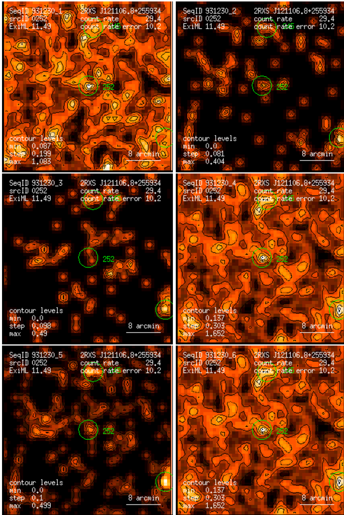
Figure 252: RASS 931230: detection 0252: band rate images, Gaussian filter: (1) PSPC channels 11 – 41, (2) 52 – 90, (3) 91 – 201, (4) 11 – 235, (5) 52 – 201, (6) 11 – 201. Broad band rates in counts/ks. Band rate contour levels in counts/ks/arcmin 2 .
