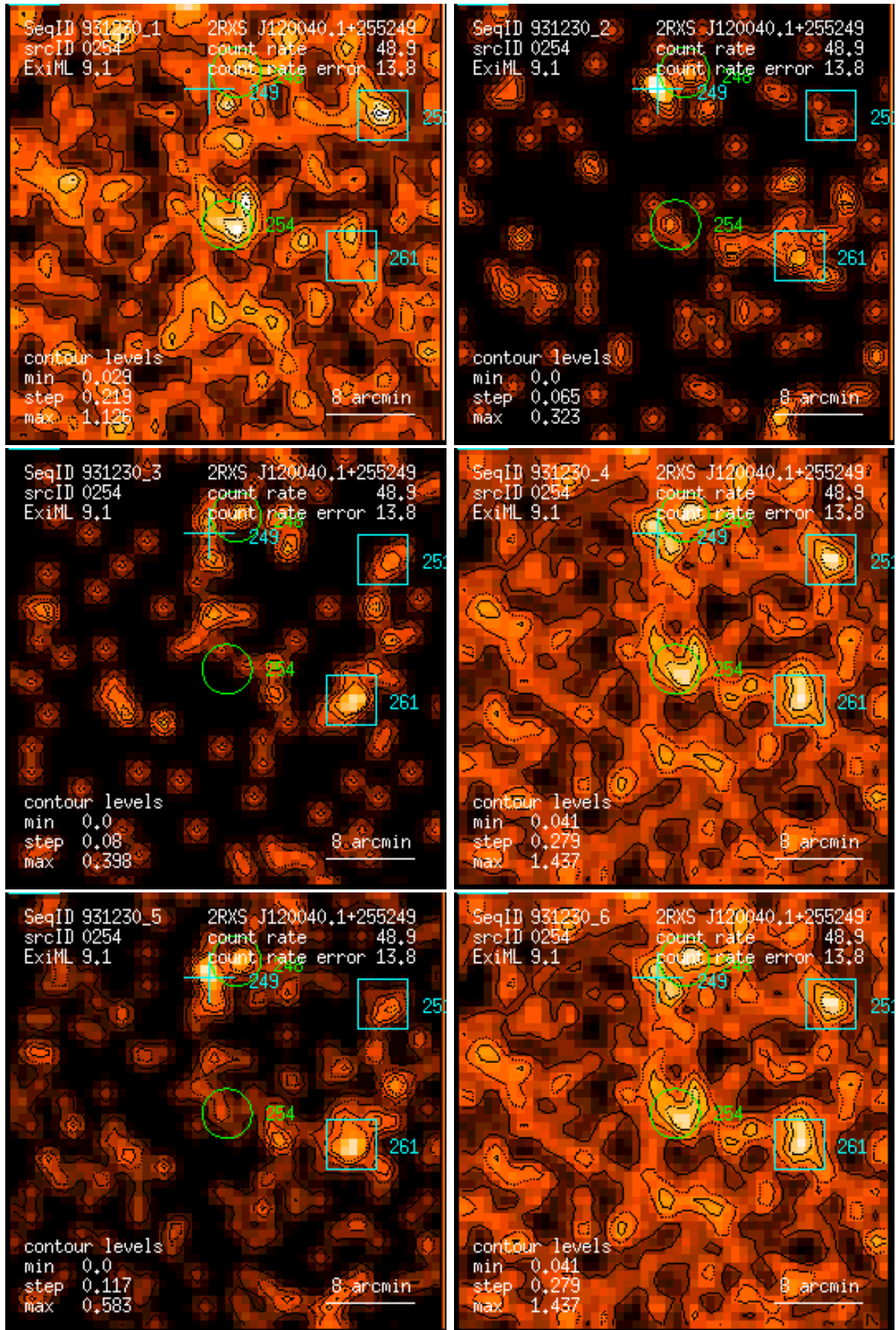
Figure 254: RASS 931230: detection 0254: band rate images, Gaussian filter: (1) PSPC channels 11 – 41, (2) 52 – 90, (3) 91 – 201, (4) 11 – 235, (5) 52 – 201, (6) 11 – 201. Broad band rates in counts/ks. Band rate contour levels in counts/ks/arcmin 2 .
