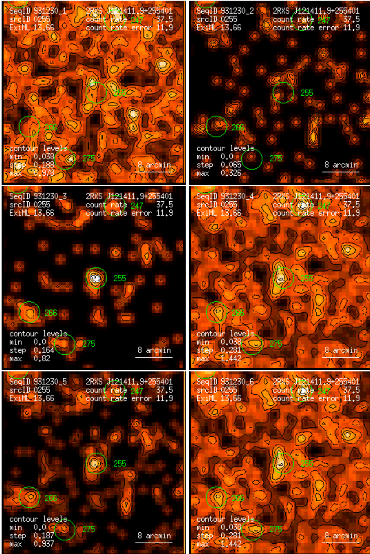
Figure 255: RASS 931230: detection 0255: band rate images, Gaussian filter: (1) PSPC channels 11 – 41, (2) 52 – 90, (3) 91 – 201, (4) 11 – 235, (5) 52 – 201, (6) 11 – 201. Broad band rates in counts/ks. Band rate contour levels in counts/ks/arcmin 2 .
