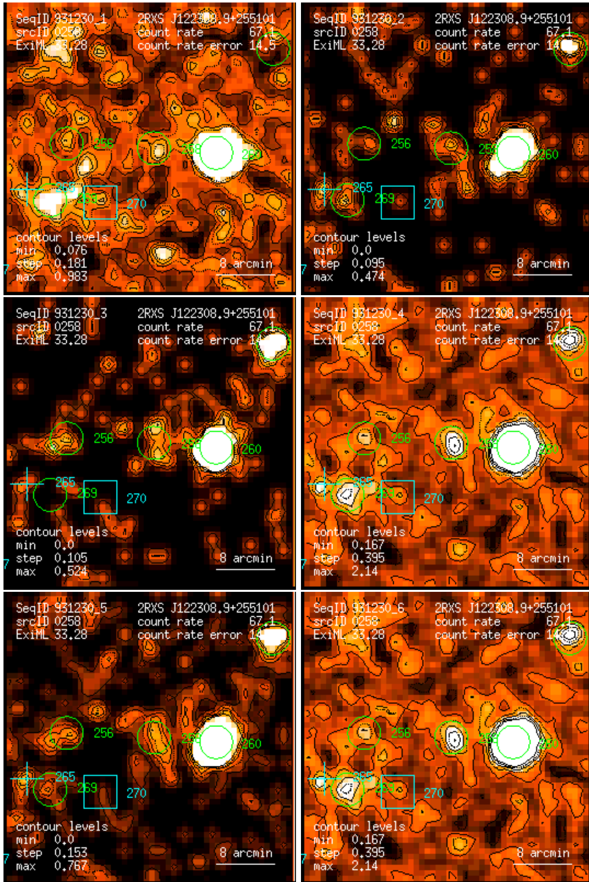
Figure 258: RASS 931230: detection 0258: band rate images, Gaussian filter: (1) PSPC channels 11 – 41, (2) 52 – 90, (3) 91 – 201, (4) 11 – 235, (5) 52 – 201, (6) 11 – 201. Broad band rates in counts/ks. Band rate contour levels in counts/ks/arcmin 2 .
