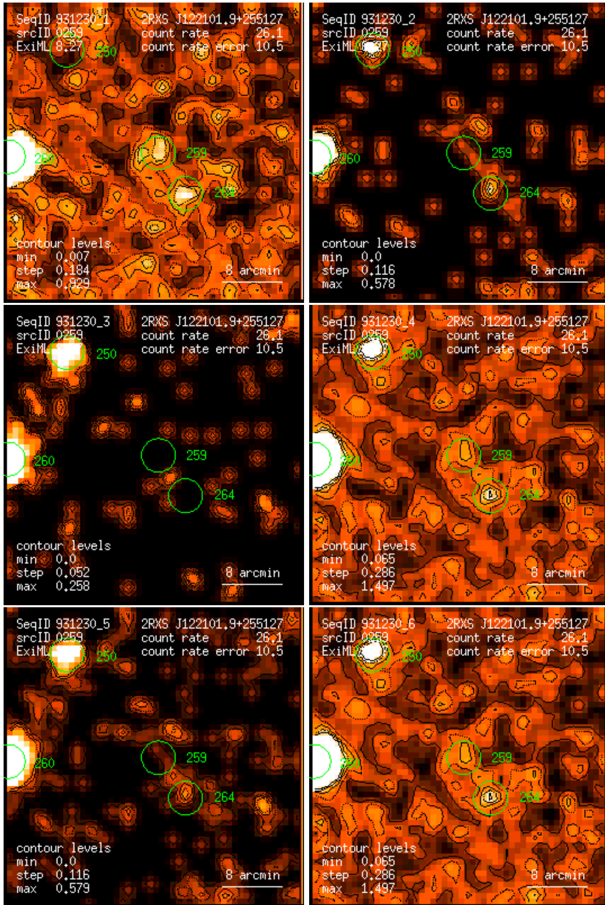
Figure 259: RASS 931230: detection 0259: band rate images, Gaussian filter: (1) PSPC channels 11 – 41, (2) 52 – 90, (3) 91 – 201, (4) 11 – 235, (5) 52 – 201, (6) 11 – 201. Broad band rates in counts/ks. Band rate contour levels in counts/ks/arcmin 2 .
