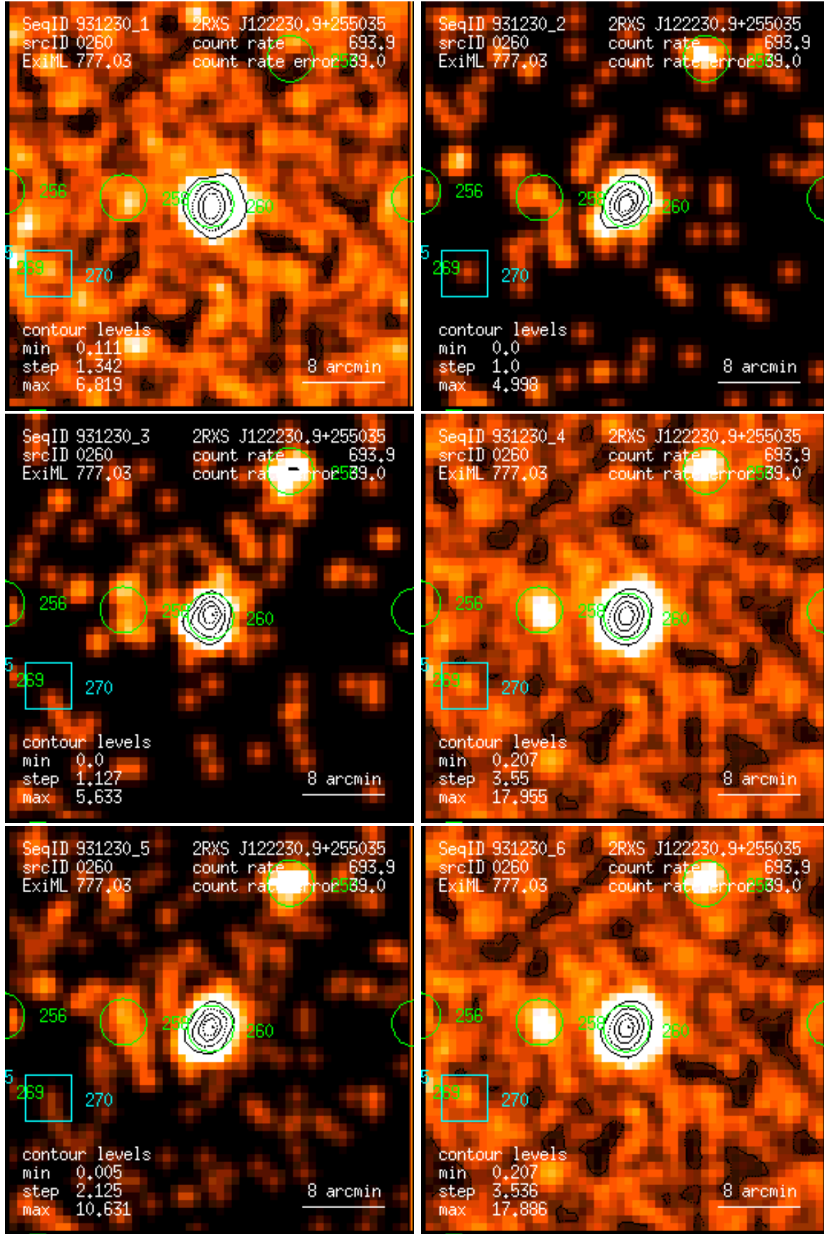
Figure 260: RASS 931230: detection 0260: band rate images, Gaussian filter: (1) PSPC channels 11 – 41, (2) 52 – 90, (3) 91 – 201, (4) 11 – 235, (5) 52 – 201, (6) 11 – 201. Broad band rates in counts/ks. Band rate contour levels in counts/ks/arcmin 2 .
