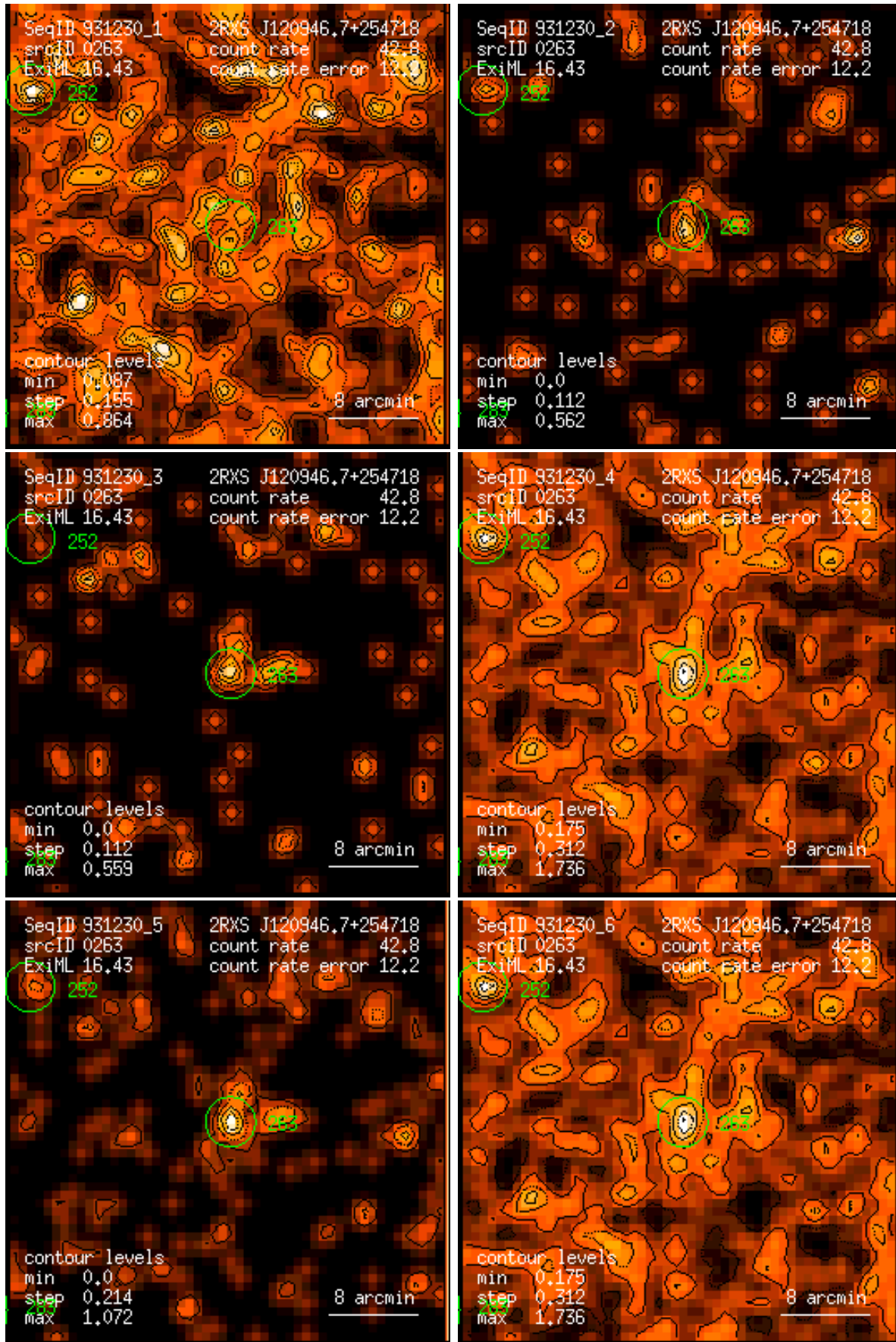
Figure 263: RASS 931230: detection 0263: band rate images, Gaussian filter: (1) PSPC channels 11 – 41, (2) 52 – 90, (3) 91 – 201, (4) 11 – 235, (5) 52 – 201, (6) 11 – 201. Broad band rates in counts/ks. Band rate contour levels in counts/ks/arcmin 2 .
