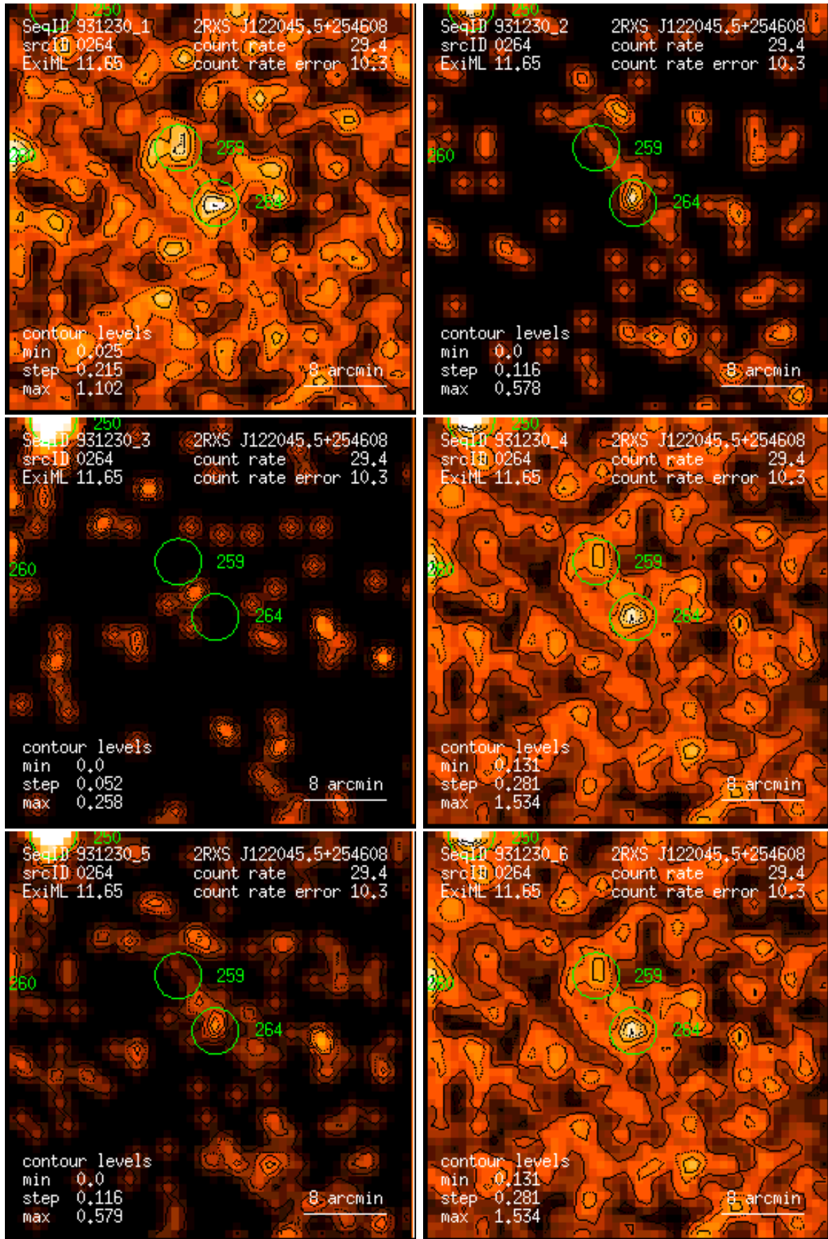
Figure 264: RASS 931230: detection 0264: band rate images, Gaussian filter: (1) PSPC channels 11 – 41, (2) 52 – 90, (3) 91 – 201, (4) 11 – 235, (5) 52 – 201, (6) 11 – 201. Broad band rates in counts/ks. Band rate contour levels in counts/ks/arcmin 2 .
