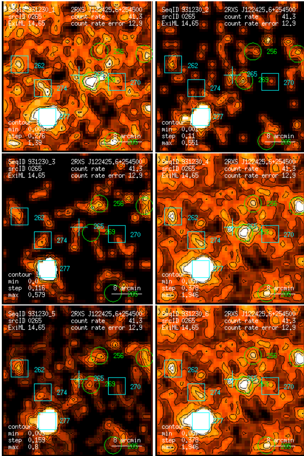
Figure 265: RASS 931230: detection 0265: band rate images, Gaussian filter: (1) PSPC channels 11 – 41, (2) 52 – 90, (3) 91 – 201, (4) 11 – 235, (5) 52 – 201, (6) 11 – 201. Broad band rates in counts/ks. Band rate contour levels in counts/ks/arcmin 2 .
